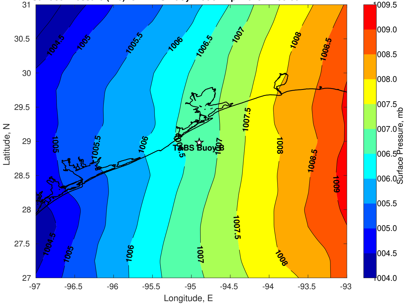
Surface Pressure (mb) for TABS Buoy B at 04-Apr-2023 12:00:00
