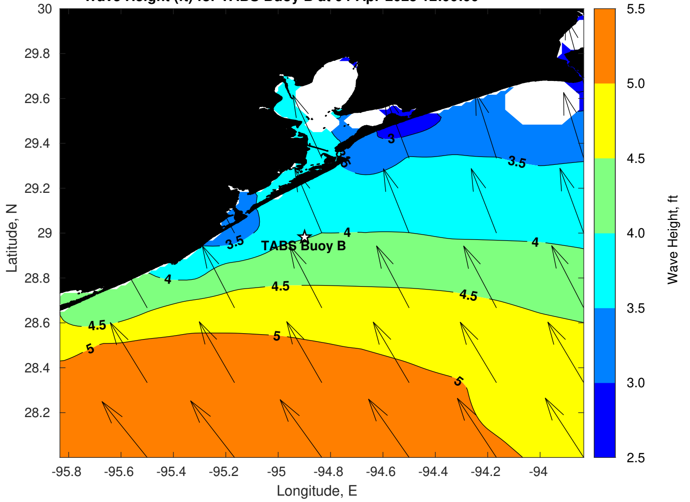
Wave Height (ft) for TABS Buoy B at 04-Apr-2023 12:00:00
