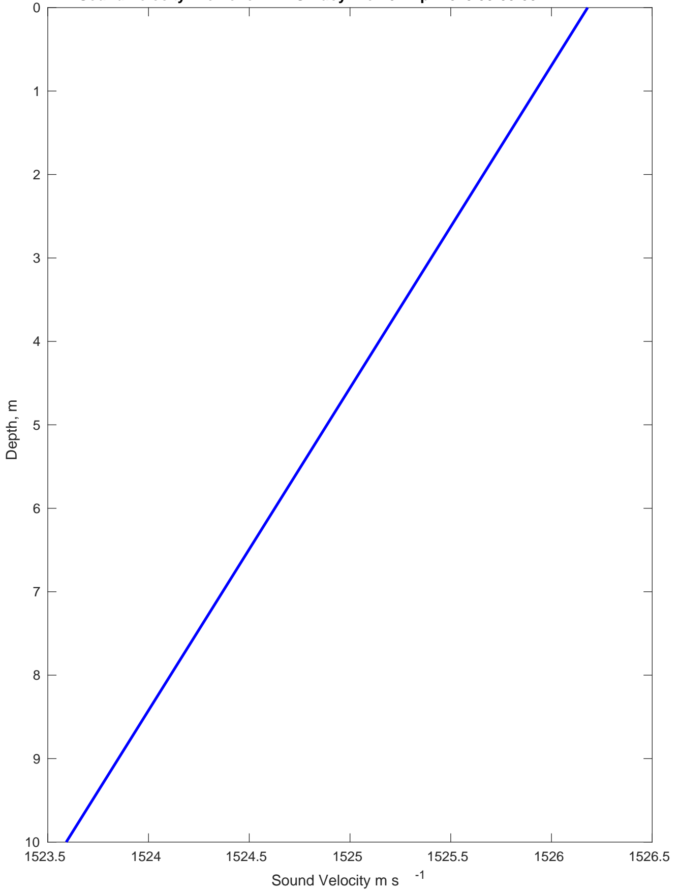
Sound Velocity Profile for TABS Buoy B on 04-Apr-2023 00:00:00
