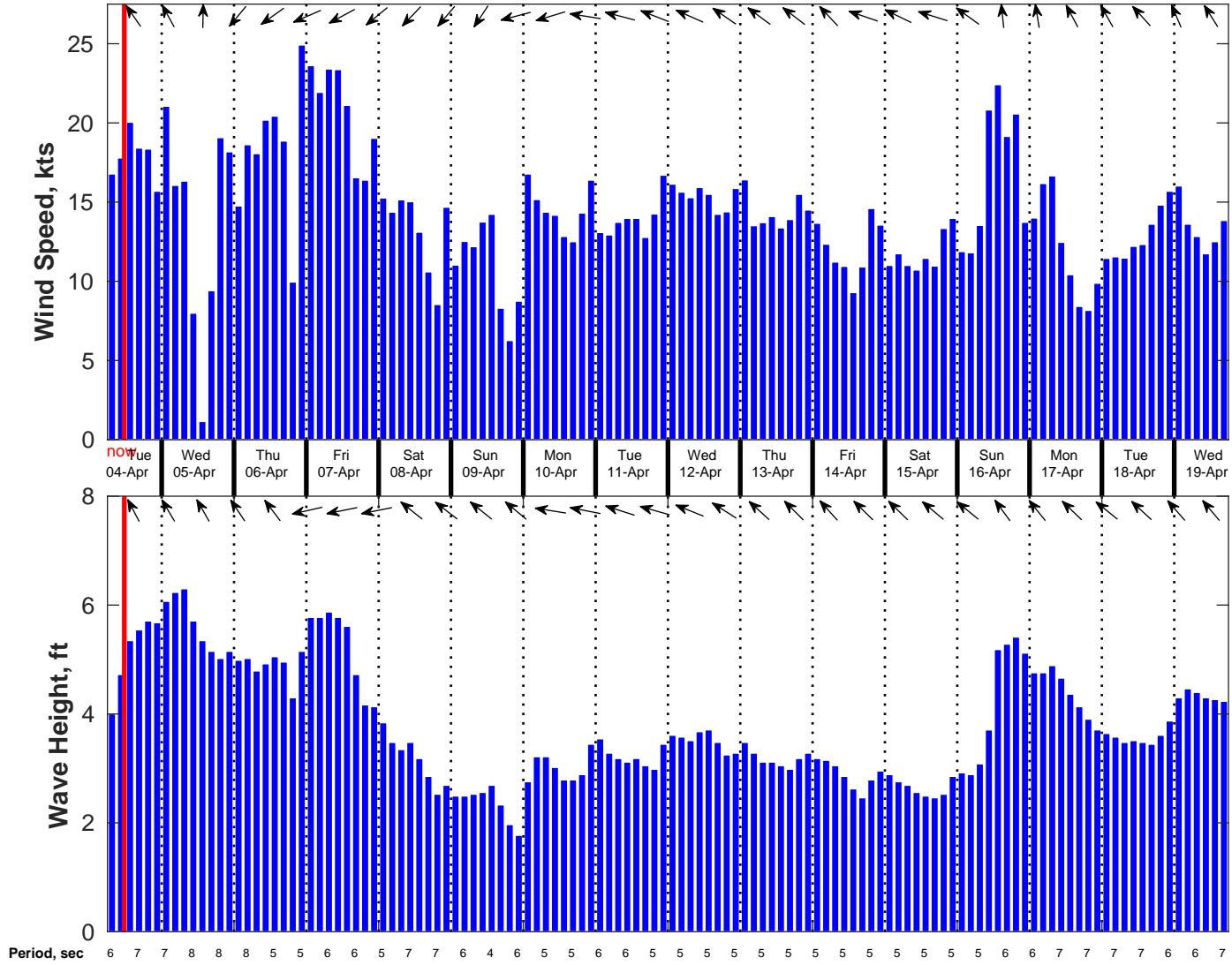
Wind & Wave Forecast for TABS Buoy B from 04-Apr-2023 06:00:00 to 20-Apr-2023 06:00:00
