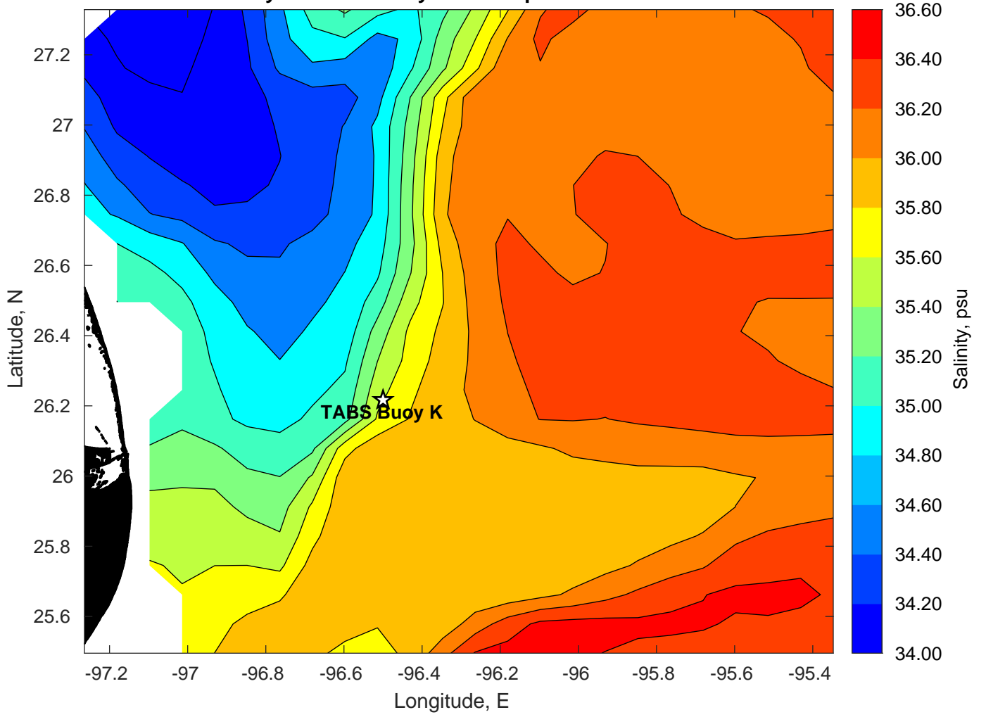
Surface Salinity for TABS Buoy K at 04-Apr-2023 00:00:00
