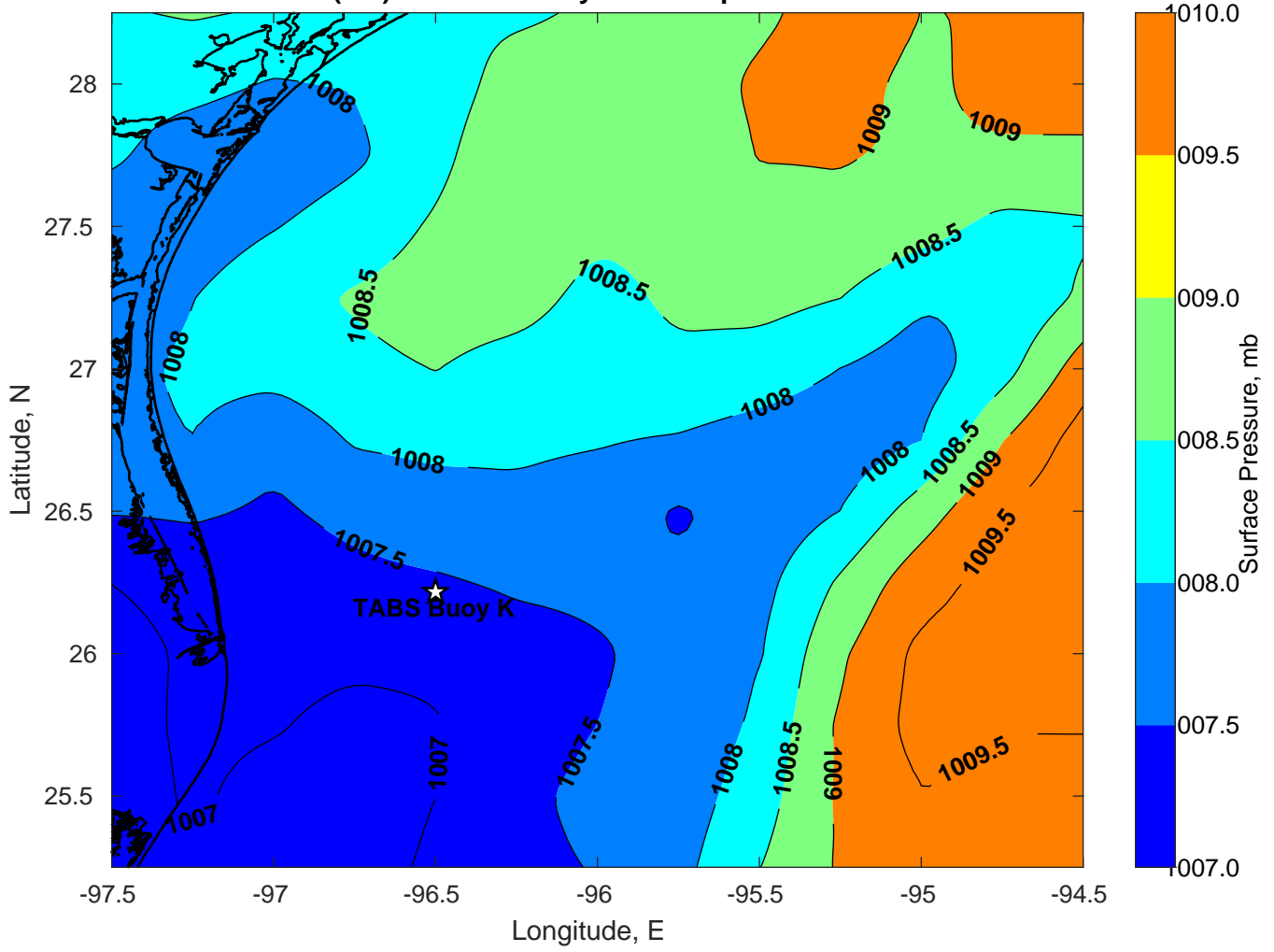
Surface Pressure (mb) for TABS Buoy K at 05-Apr-2023 12:00:00
