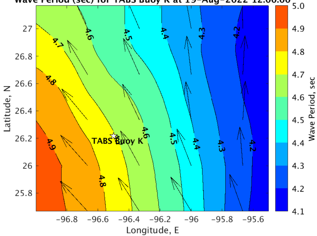
Wave Period (sec) for TABS Buoy K at 19-Aug-2022 12:00:00
