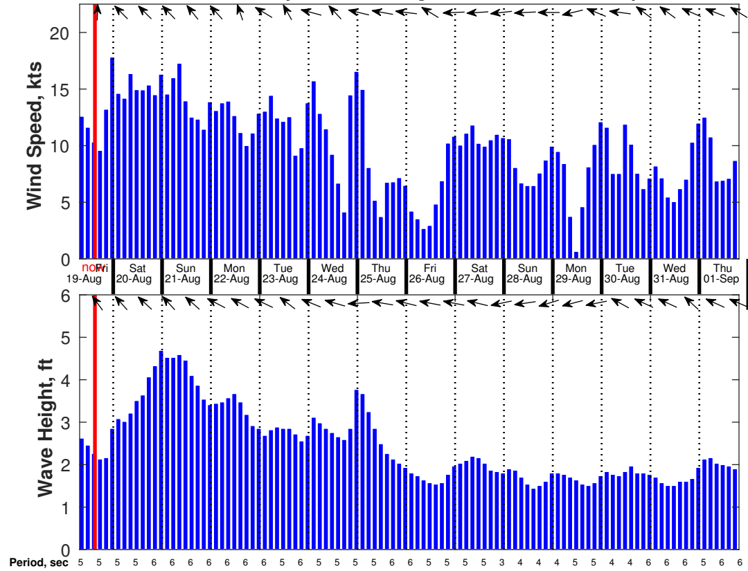
Wind & Wave Forecast for TABS Buoy K from 19-Aug-2022 07:00:00 to 02-Sep-2022 01:00:00
