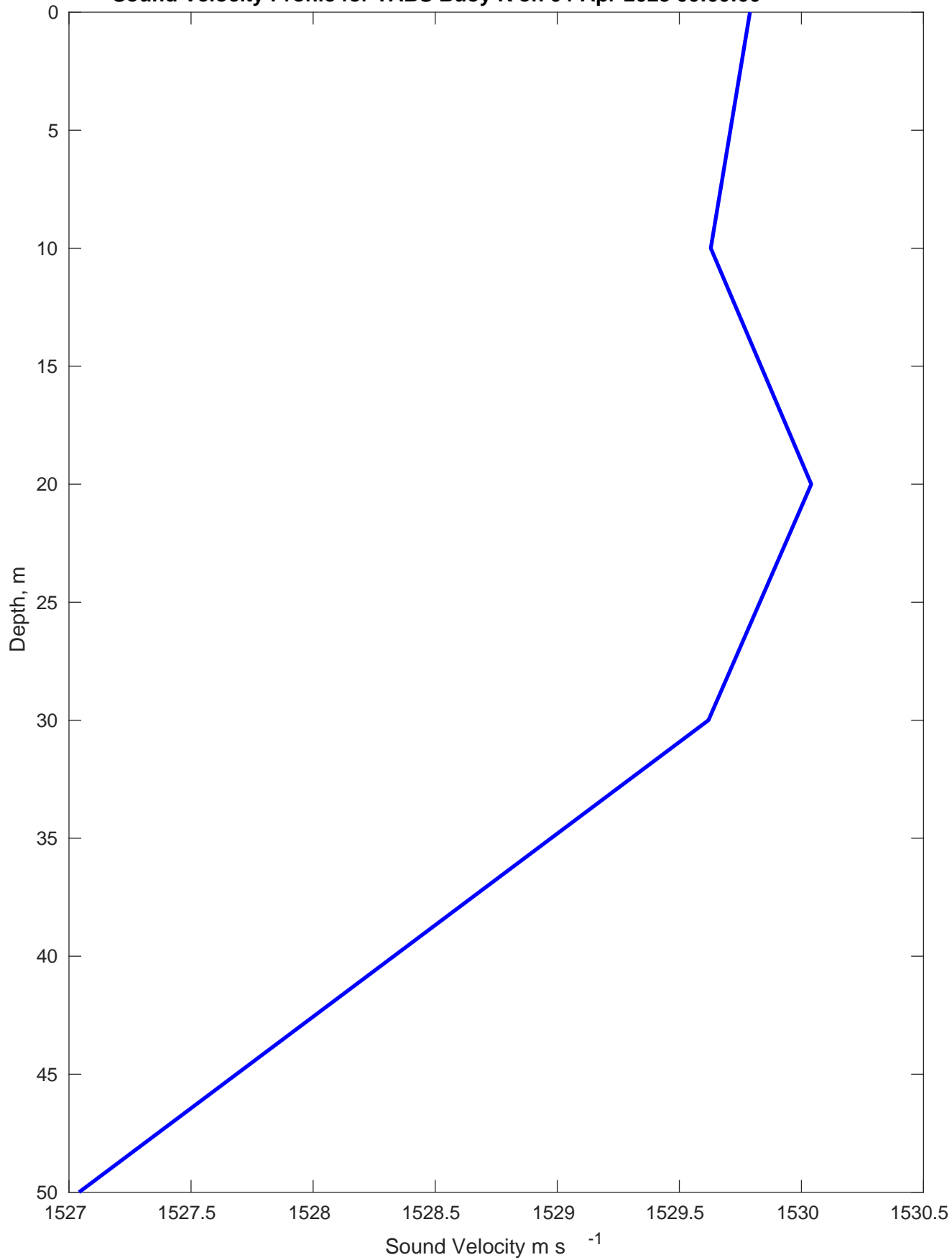
Sound Velocity Profile for TABS Buoy K on 04-Apr-2023 00:00:00
