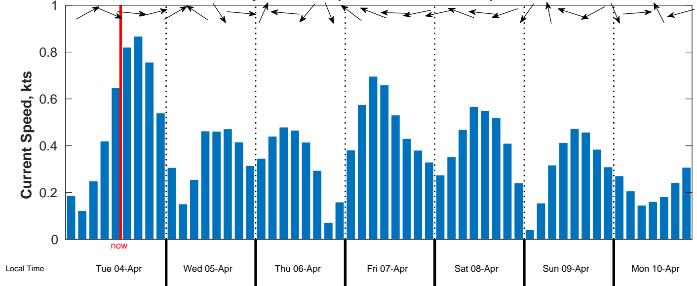
Current Forecast for TABS Buoy K from 04-Apr-2023 00:00:00 to 11-Apr-2023 00:00:00
