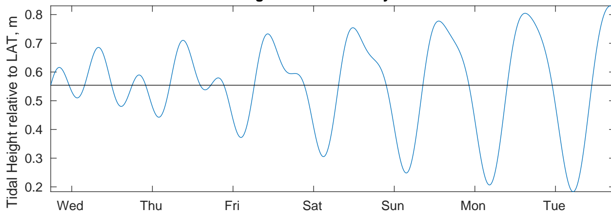
Tidal Currents and Heights for TABS Buoy K at 20230404
