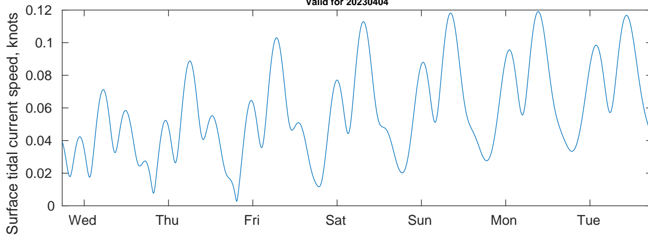
Tidal Currents and Heights for TABS Buoy K at 20230404
