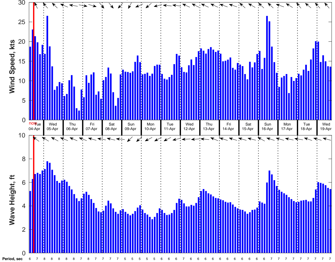
Wind & Wave Forecast for TABS Buoy K from 04-Apr-2023 06:00:00 to 20-Apr-2023 06:00:00
