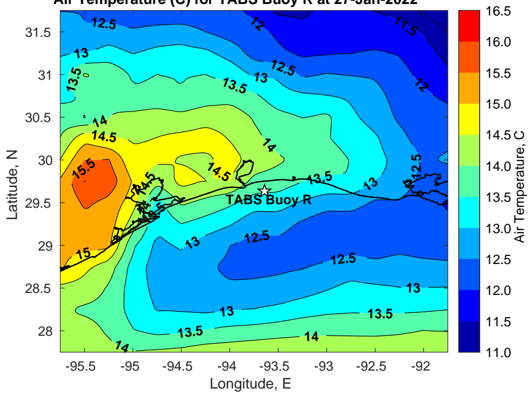
Air Temperature (C) for TABS Buoy R at 27-Jan-2022
