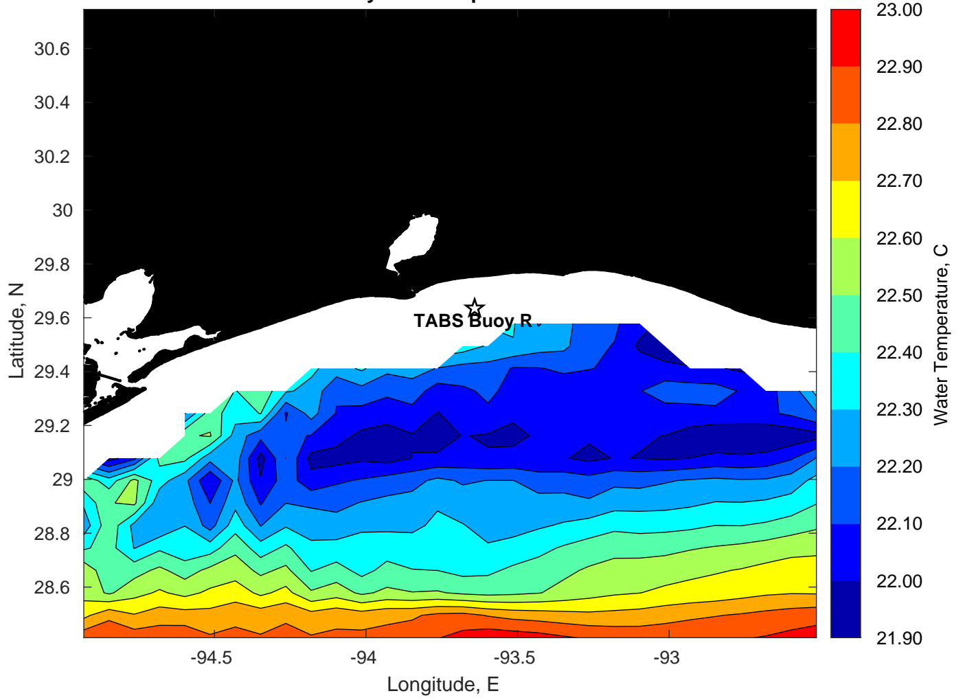
SST for TABS Buoy R at 04-Apr-2023 00:00:00
