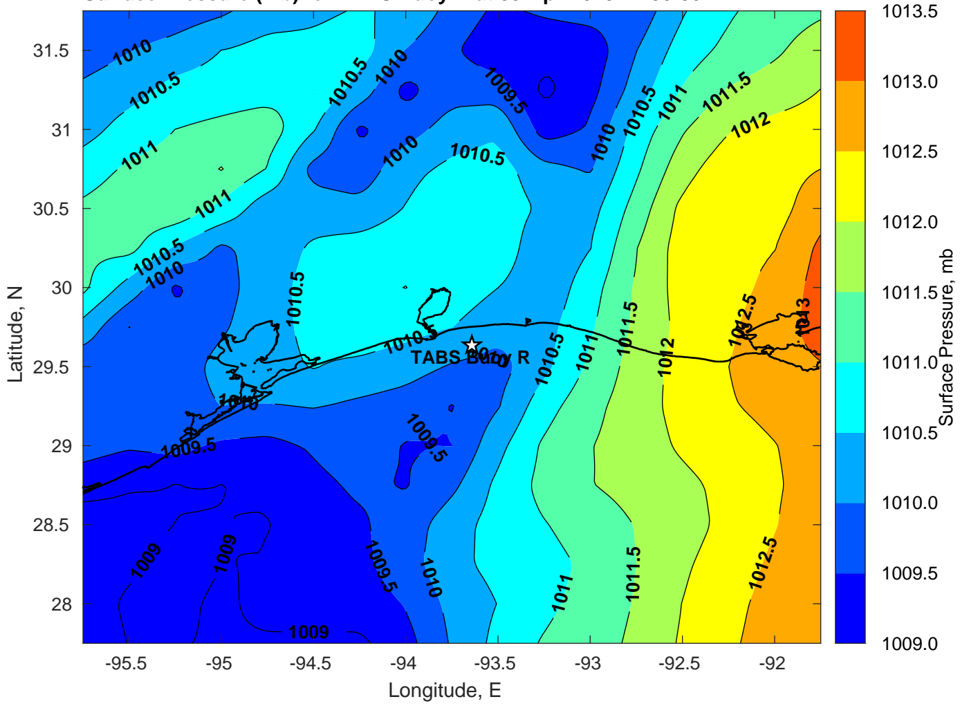
Surface Pressure (mb) for TABS Buoy R at 05-Apr-2023 12:00:00
