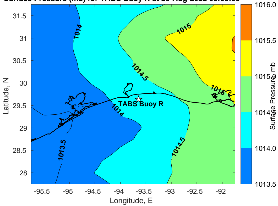
Surface Pressure (mb) for TABS Buoy R at 20-Aug-2022 09:00:00
