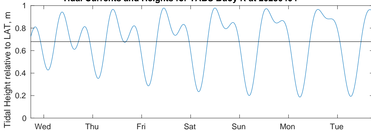
Tidal Currents and Heights for TABS Buoy R at 20230404
