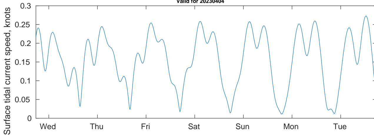
Tidal Currents and Heights for TABS Buoy R at 20230404
