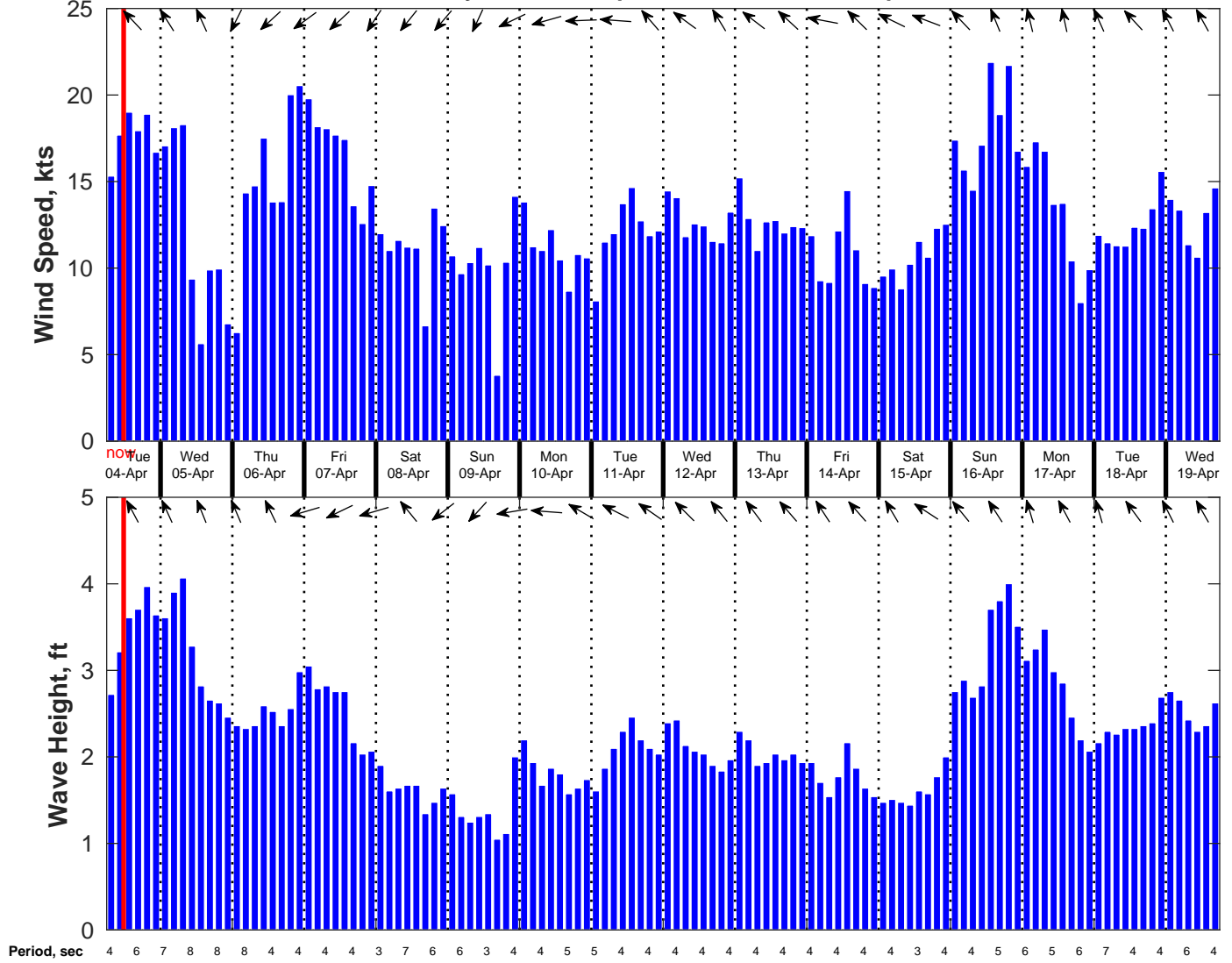
Wind & Wave Forecast for TABS Buoy R from 04-Apr-2023 06:00:00 to 20-Apr-2023 06:00:00
