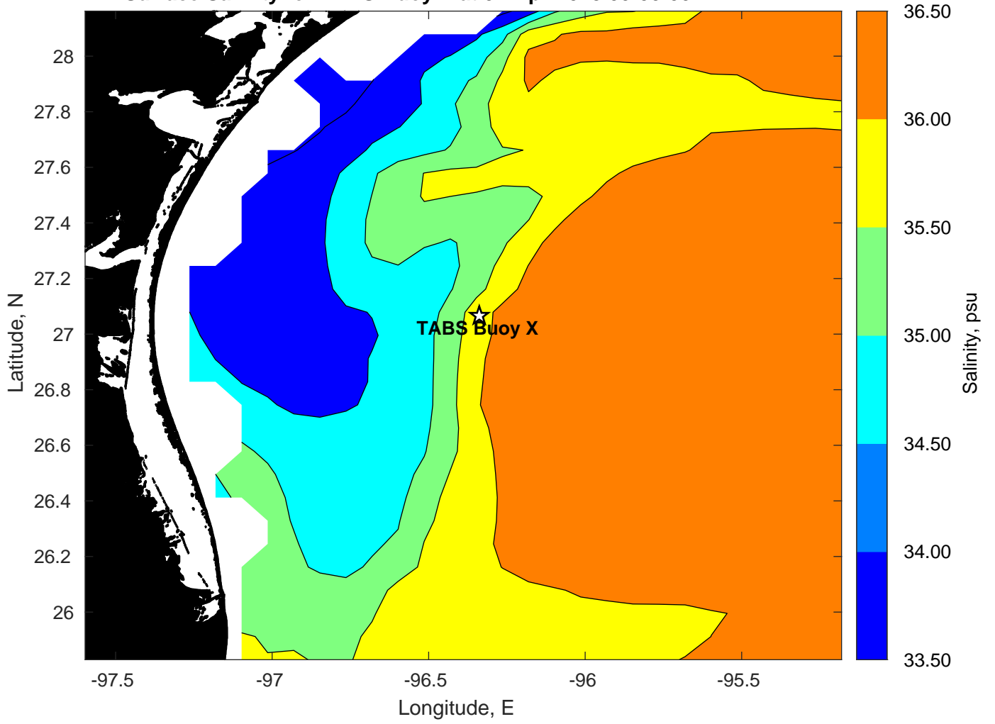
Surface Salinity for TABS Buoy X at 04-Apr-2023 00:00:00
