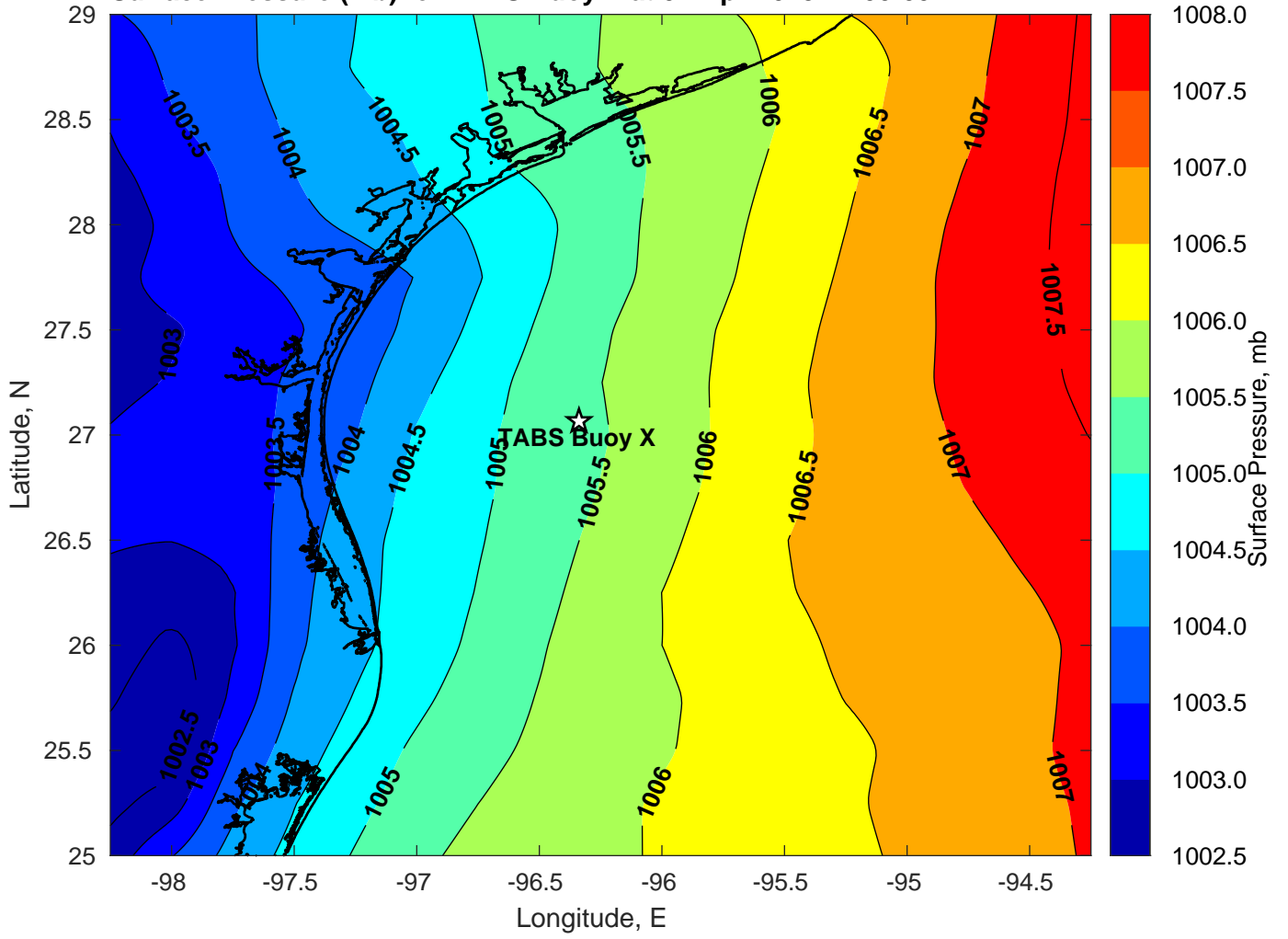
Surface Pressure (mb) for TABS Buoy X at 04-Apr-2023 12:00:00
