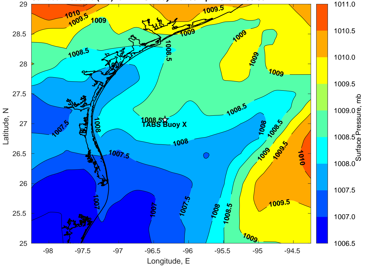
Surface Pressure (mb) for TABS Buoy X at 05-Apr-2023 12:00:00
