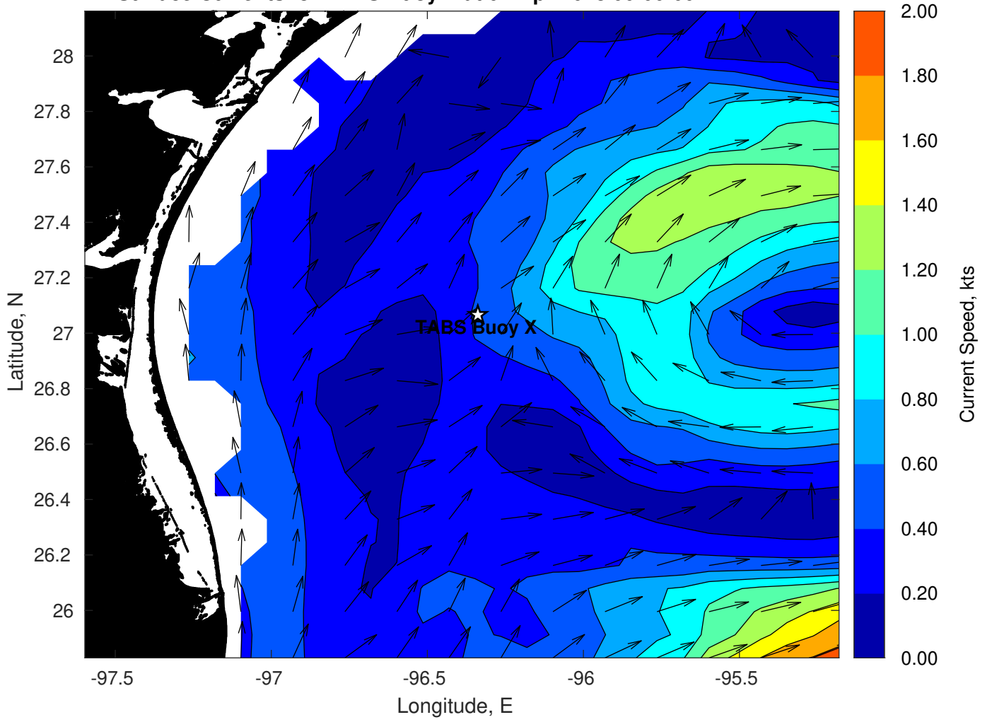
Surface Currents for TABS Buoy X at 04-Apr-2023 00:00:00
