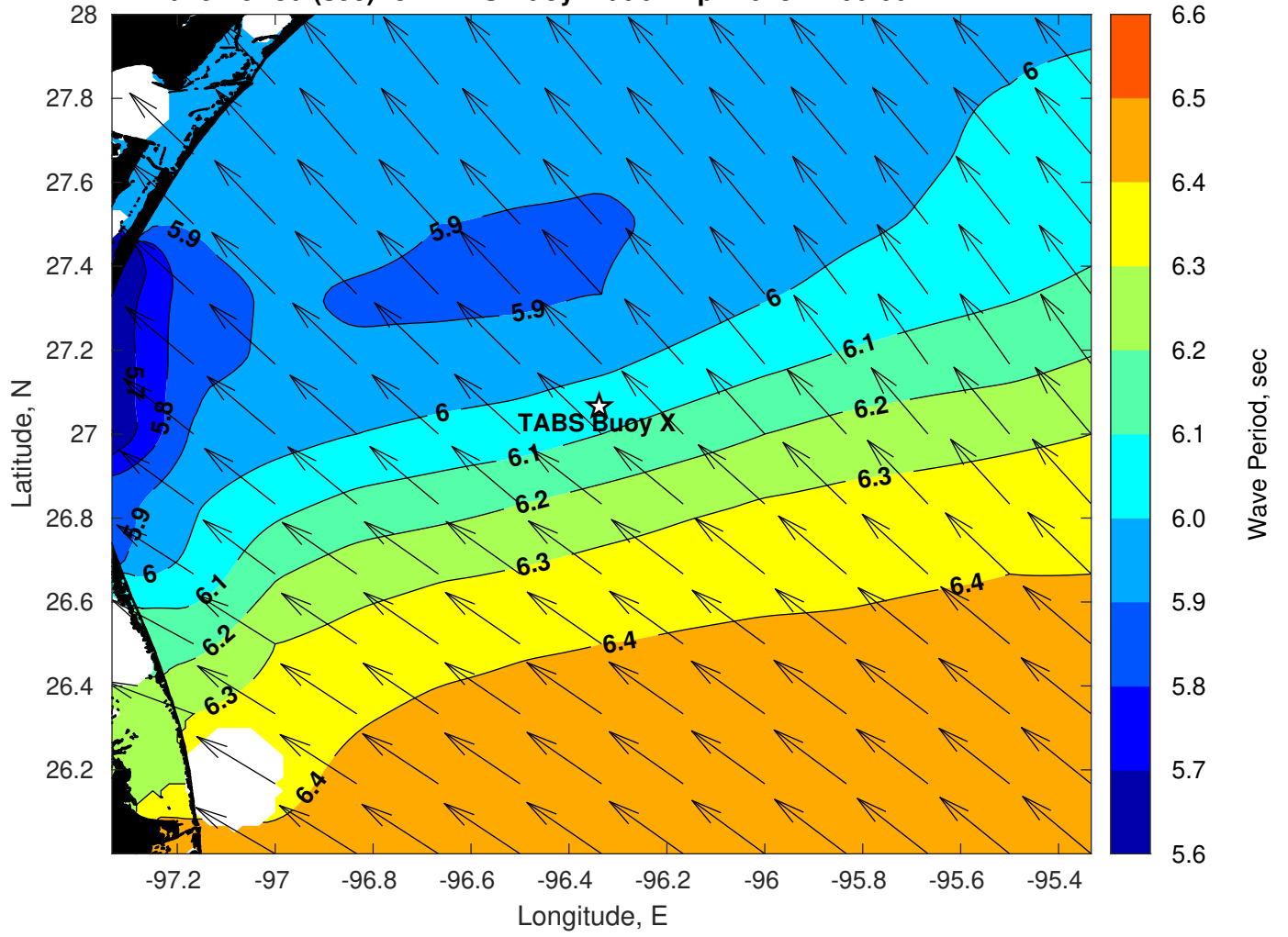
Wave Period (sec) for TABS Buoy X at 04-Apr-2023 12:00:00
