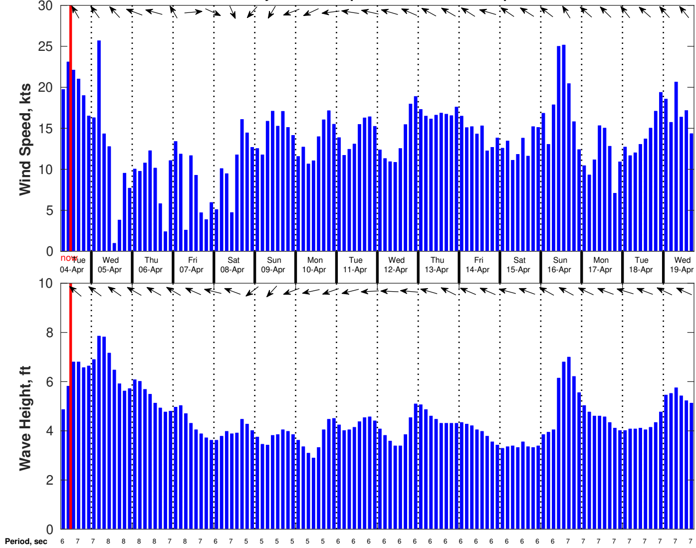
Wind & Wave Forecast for TABS Buoy X from 04-Apr-2023 06:00:00 to 20-Apr-2023 06:00:00
