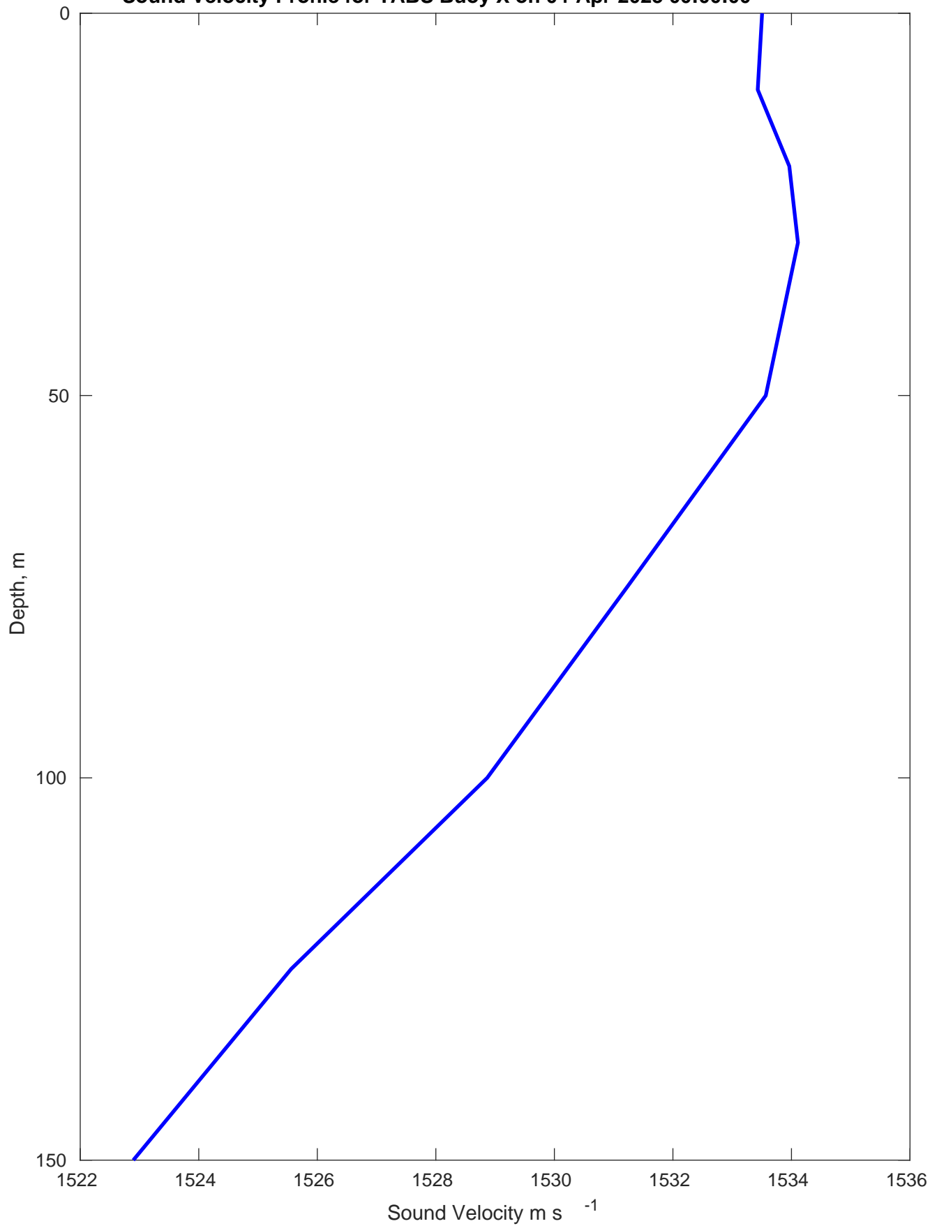
Sound Velocity Profile for TABS Buoy X on 04-Apr-2023 00:00:00
