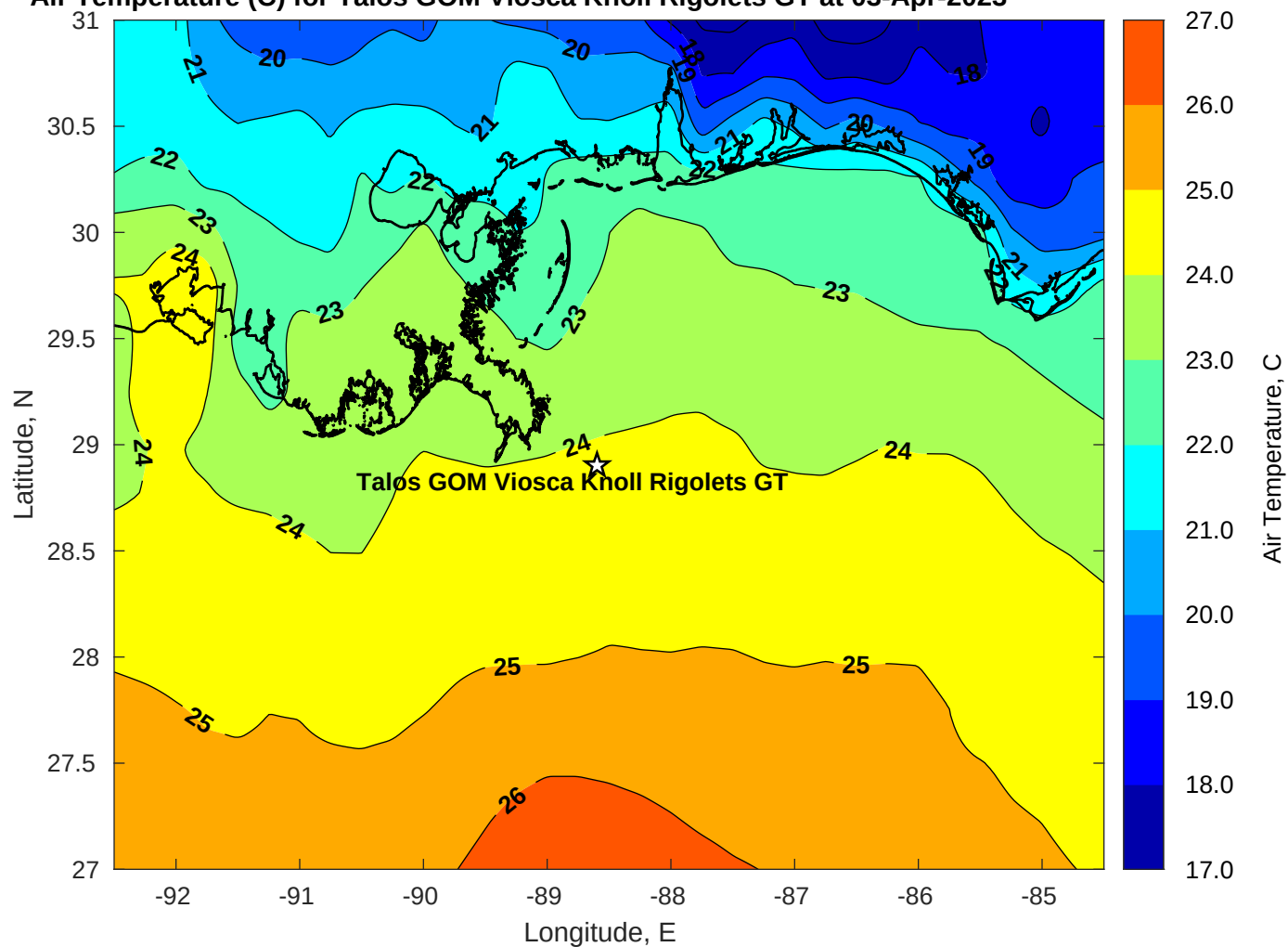
Air Temperature (C) for Talos GOM Viosca Knoll Rigolets GT at 03-Apr-2023
