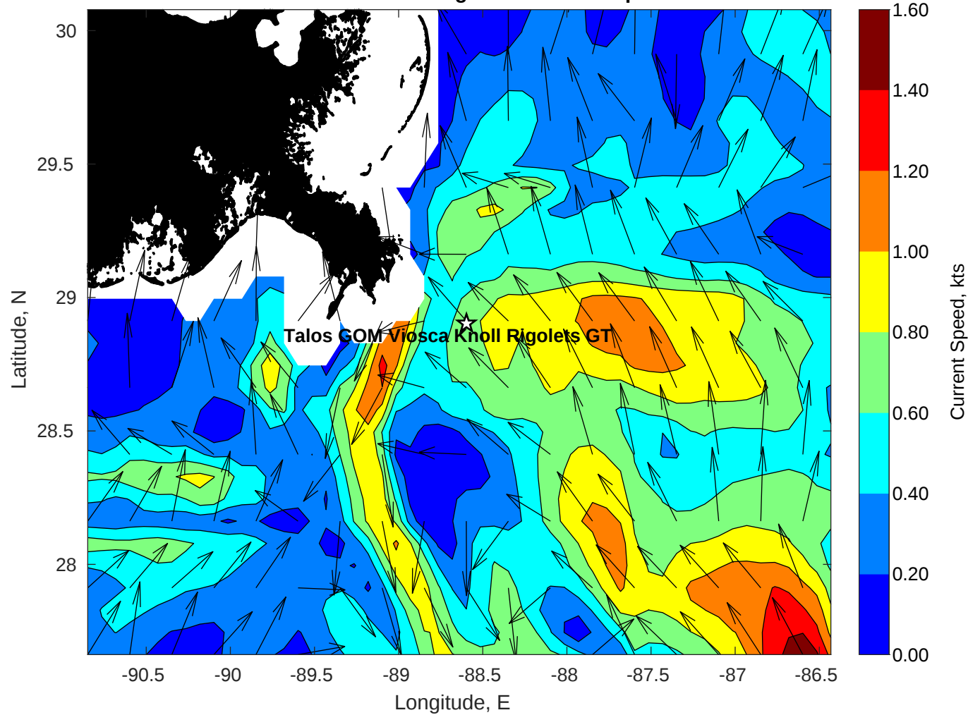
Surface Currents for Talos GOM Viosca Knoll Rigolets GT at 03-Apr-2023 00:00:00
