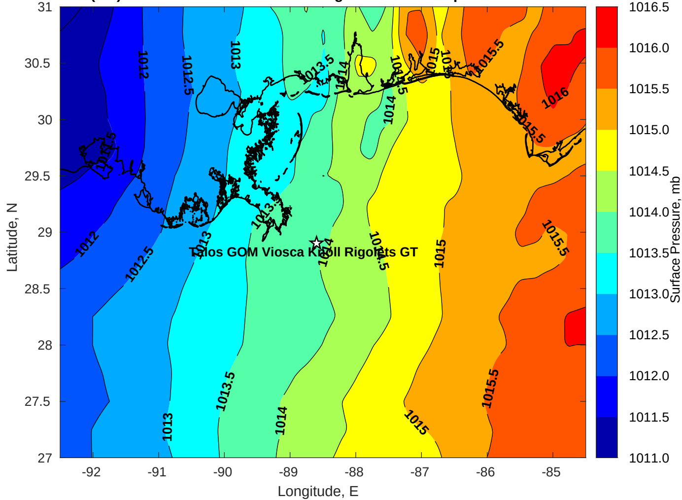
Surface Pressure (mb) for Talos GOM Viosca Knoll Rigolets GT at 03-Apr-2023 06:00:00
