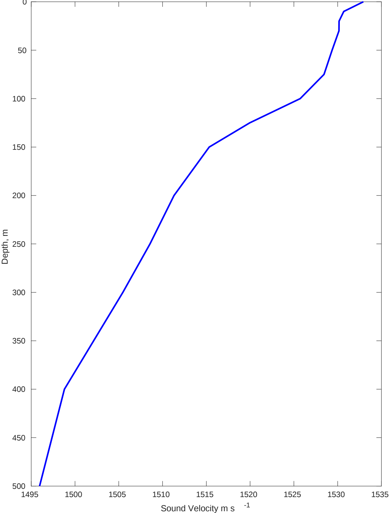
Sound Velocity Profile for Talos GOM Viosca Knoll Rigolets GT on 03-Apr-2023 00:00:00
