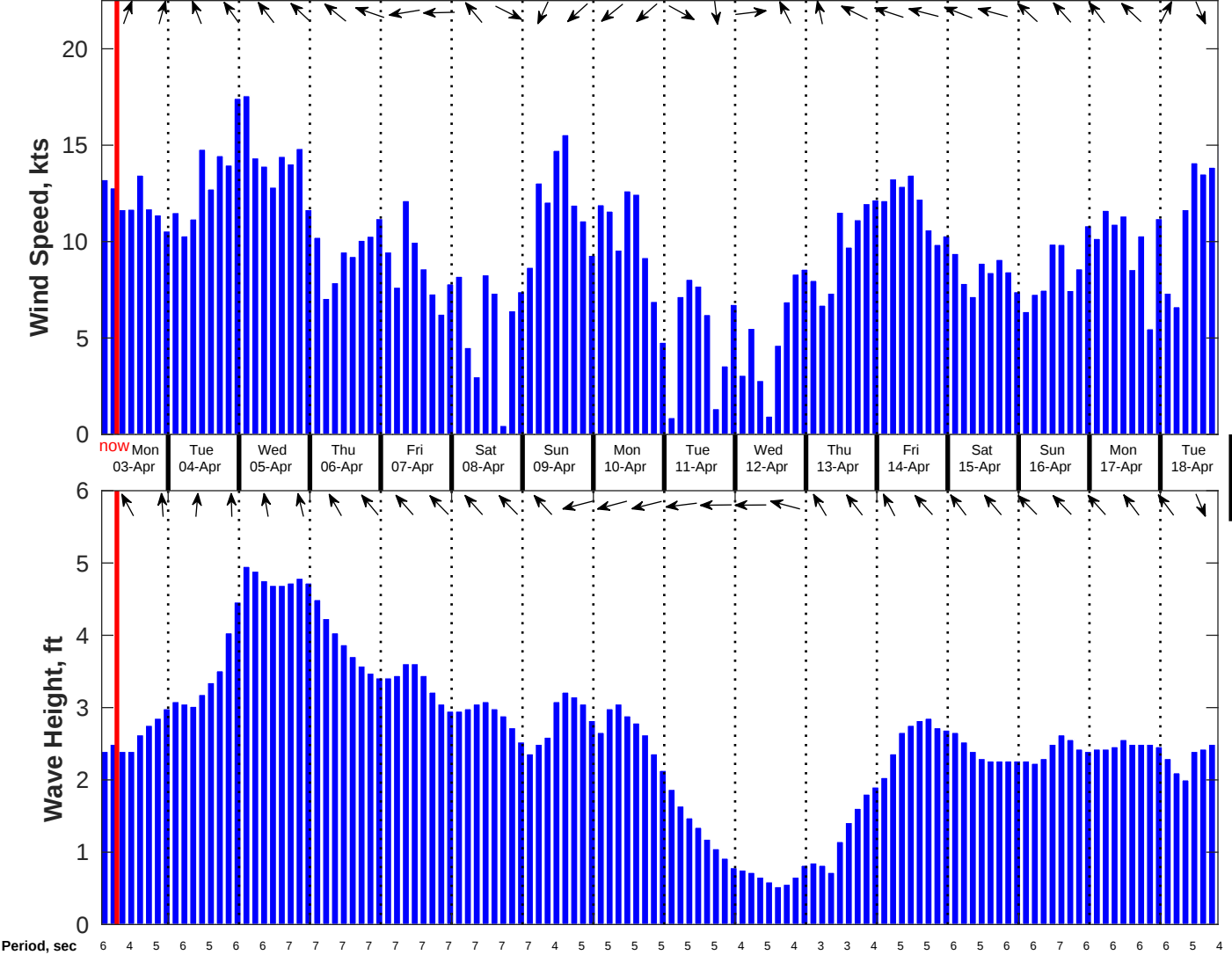
Wind & Wave Forecast for Talos GOM Viosca Knoll Rigolets GT from 03-Apr-2023 01:00:00 to 19-Apr-2023 01:00:00
