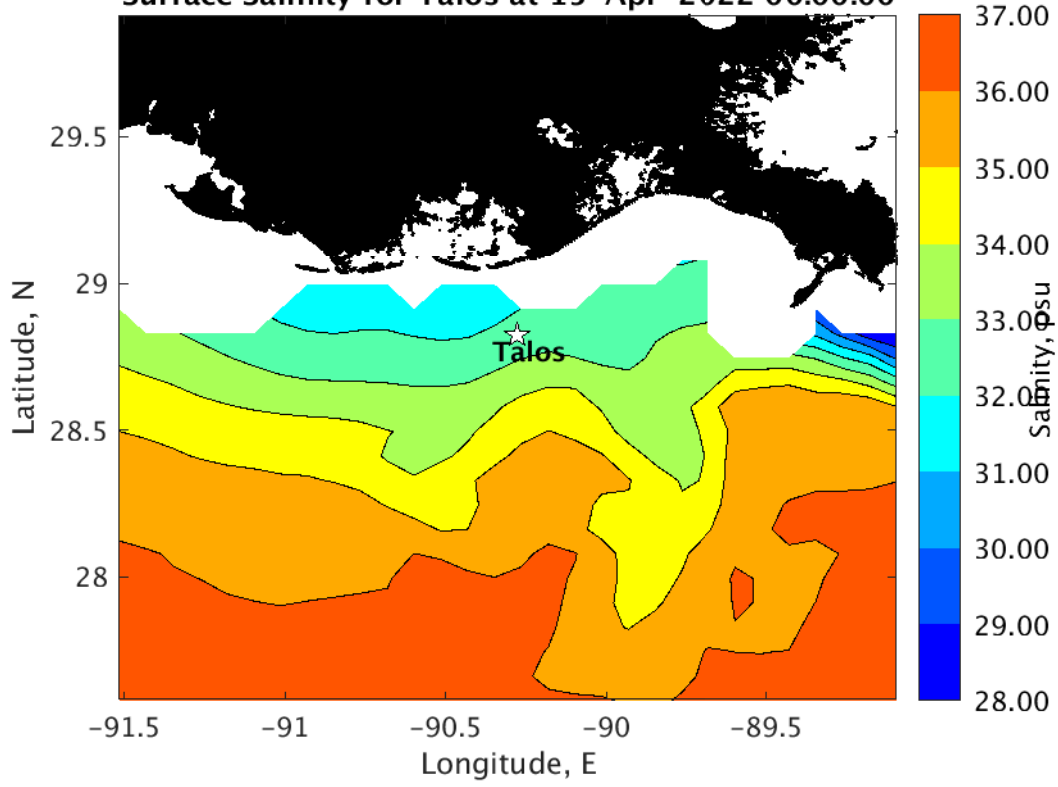
Surface Salinity for Talos at 15-Apr-2022 00:00:00
