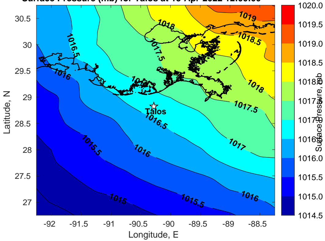
Surface Pressure (mb) for Talos at 15-Apr-2022 12:00:00
