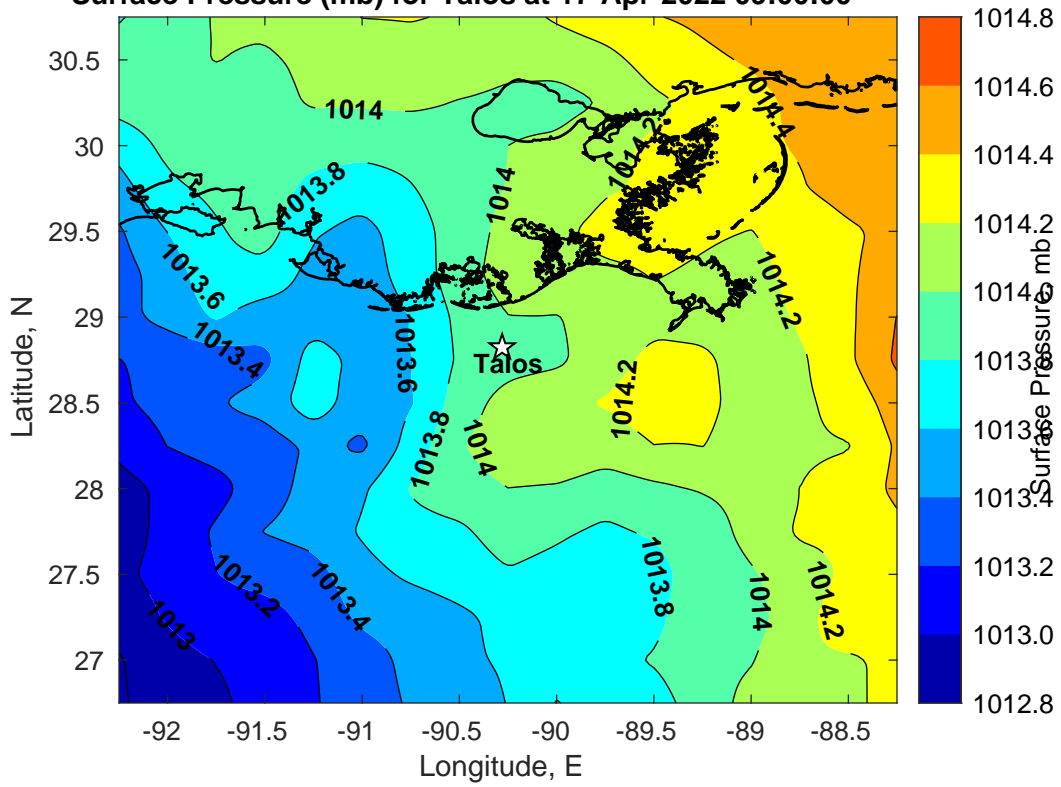
Surface Pressure (mb) for Talos at 17-Apr-2022 09:00:00
