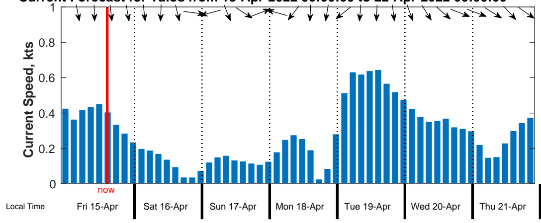
Current Forecast for Talos from 15-Apr-2022 00:00:00 to 22-Apr-2022 00:00:00
