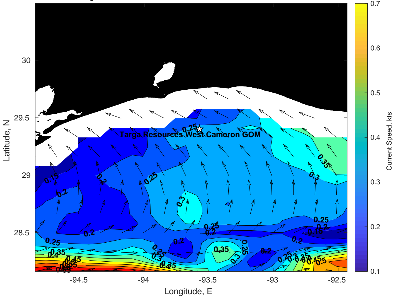
Surface Currents for Targa Resources West Cameron GOM at 05-Jun-2024 00:00:00
