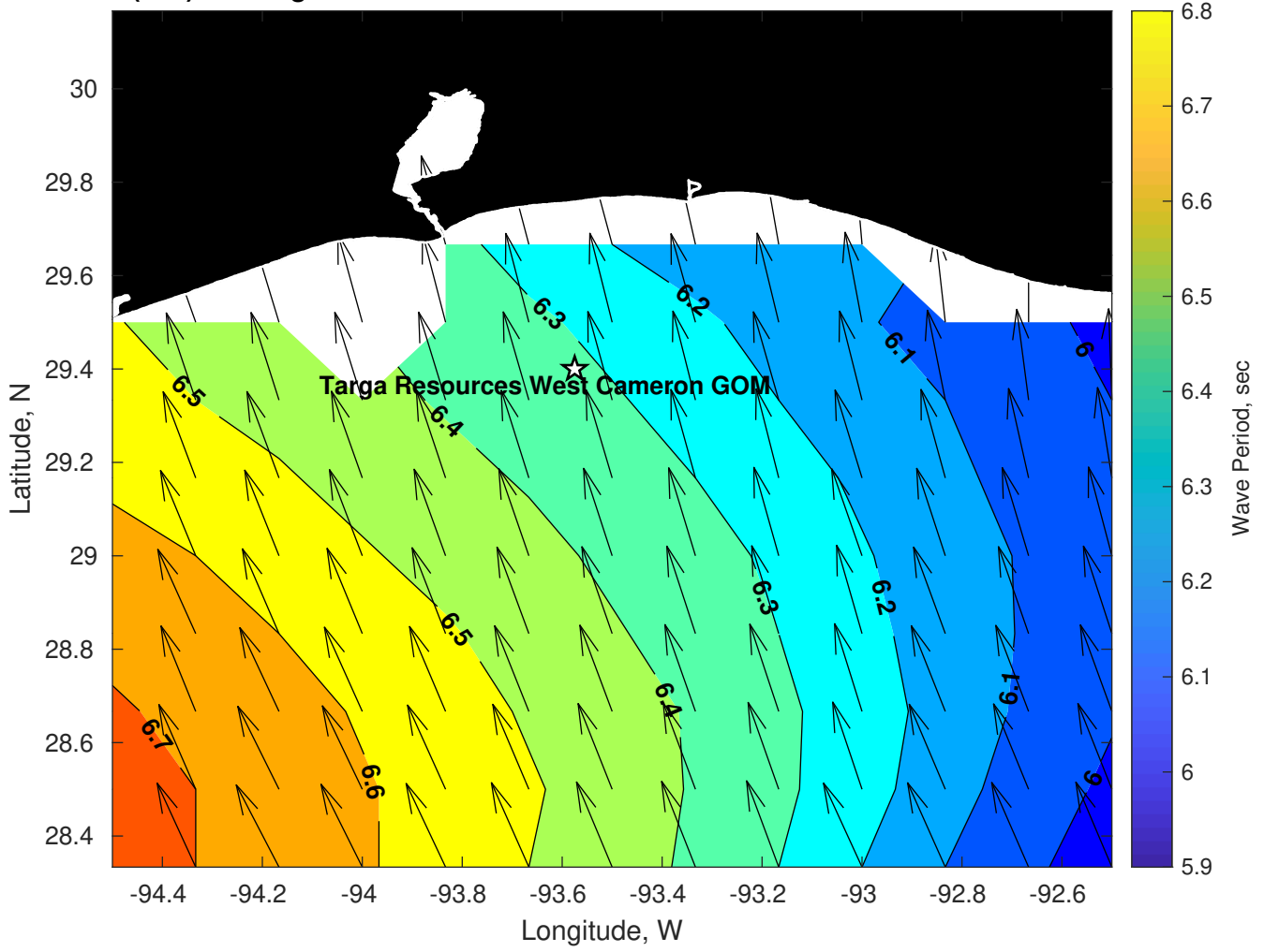
Wave Period (sec) for Targa Resources West Cameron GOM at 05-Jun-2024 18:00:00
