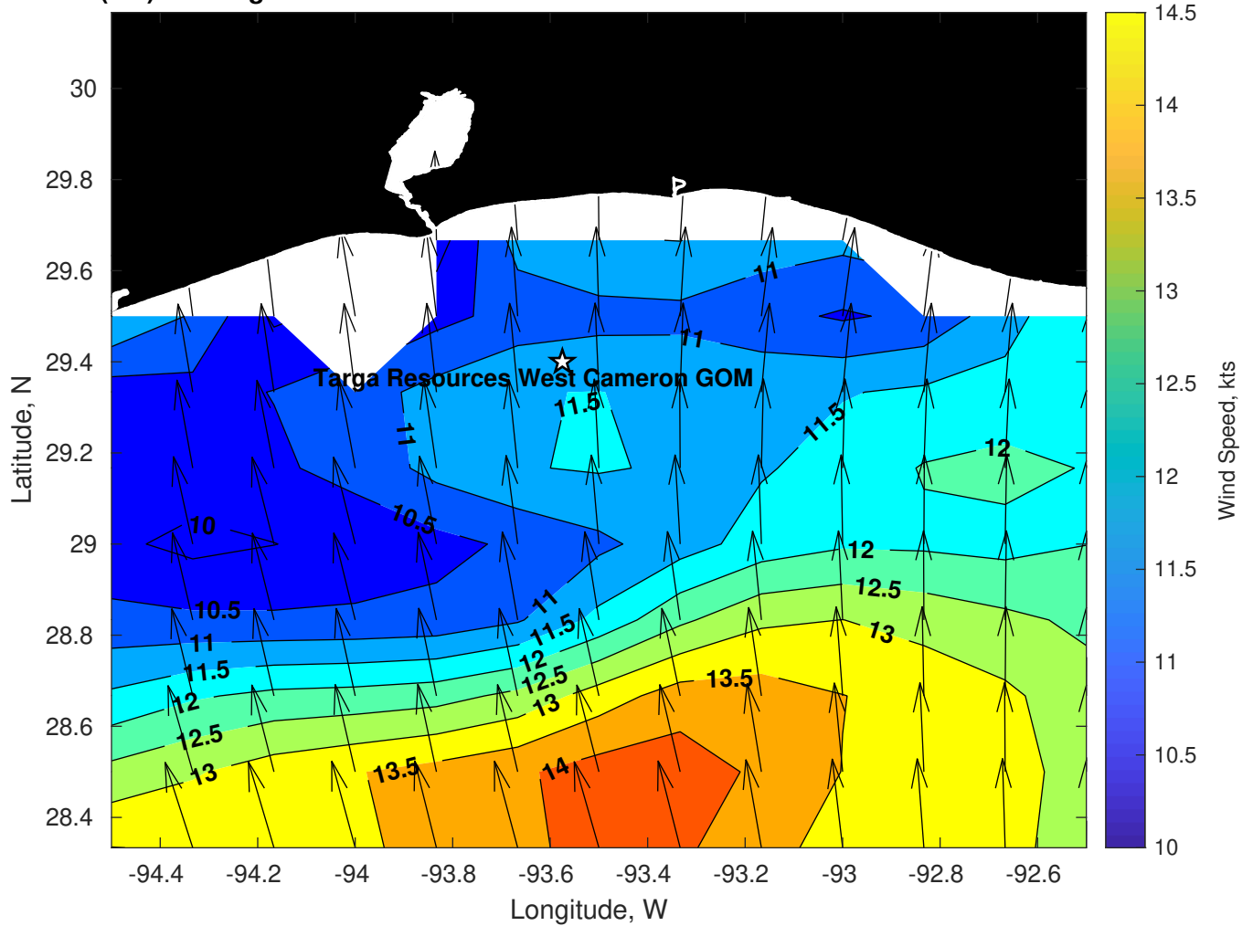
Winds (kts) for Targa Resources West Cameron GOM at 05-Jun-2024 18:00:00
