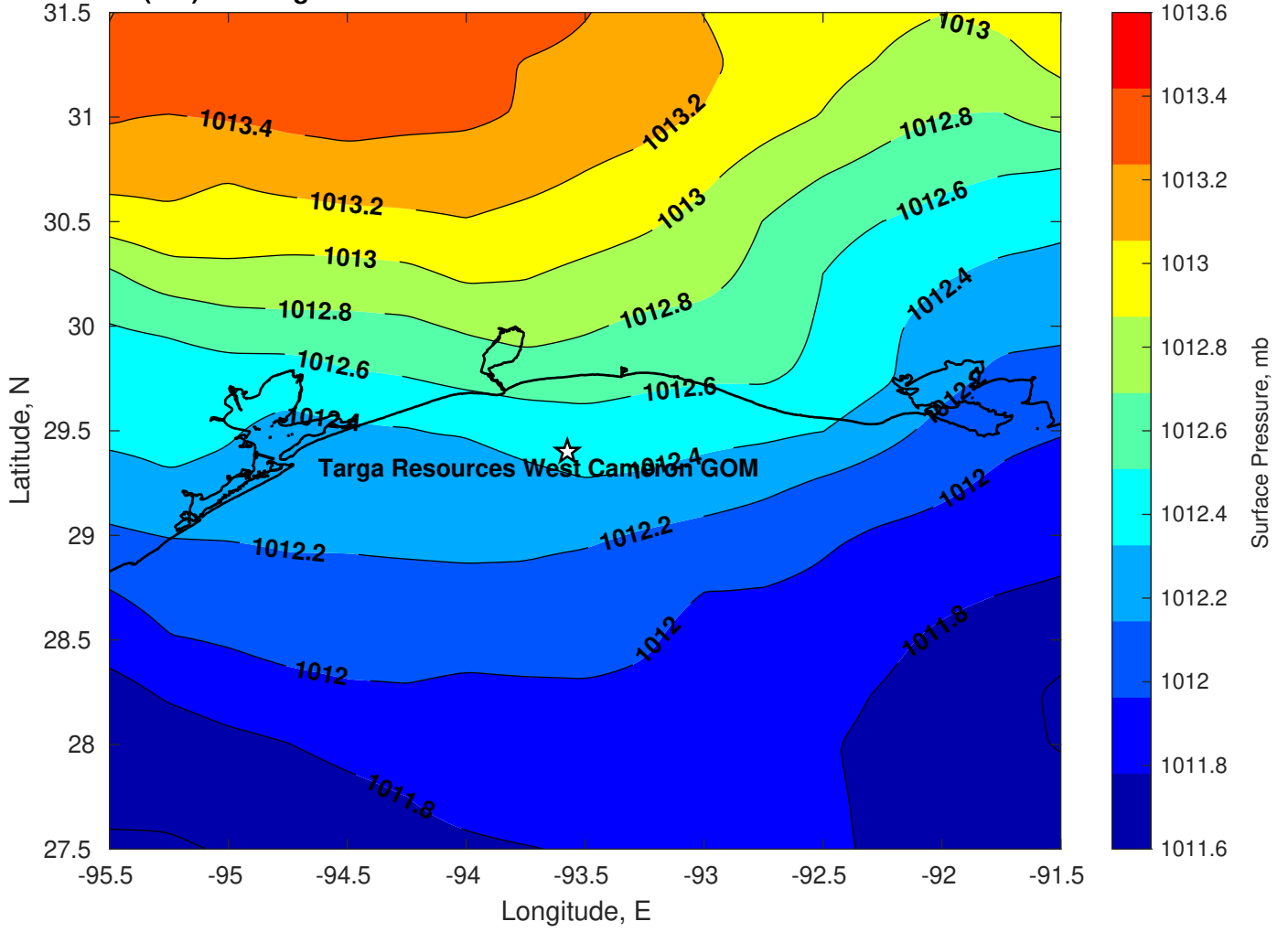
Surface Pressure (mb) for Targa Resources West Cameron GOM at 07-Jun-2024 12:00:00
