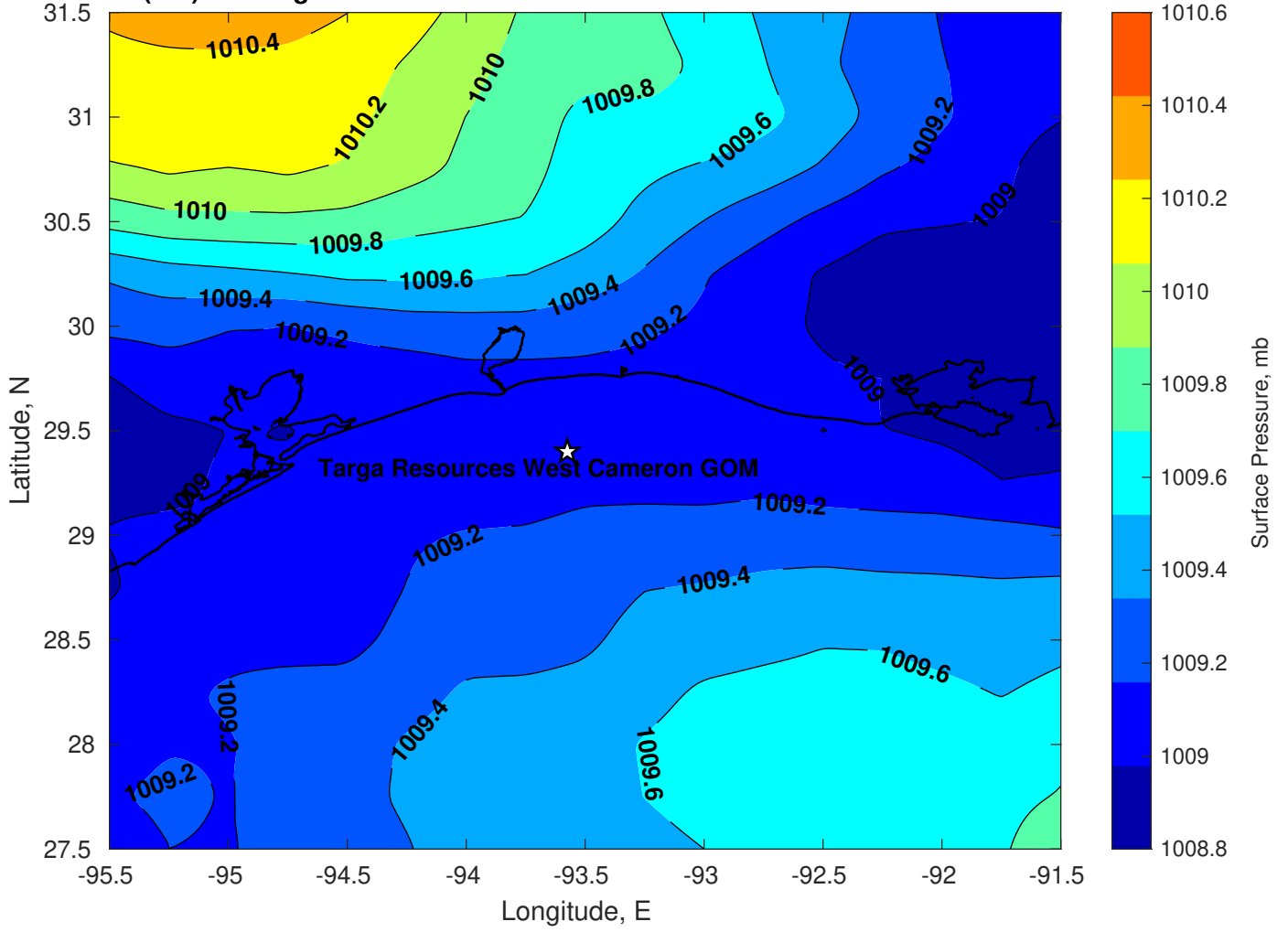
Surface Pressure (mb) for Targa Resources West Cameron GOM at 06-Jun-2024 12:00:00
