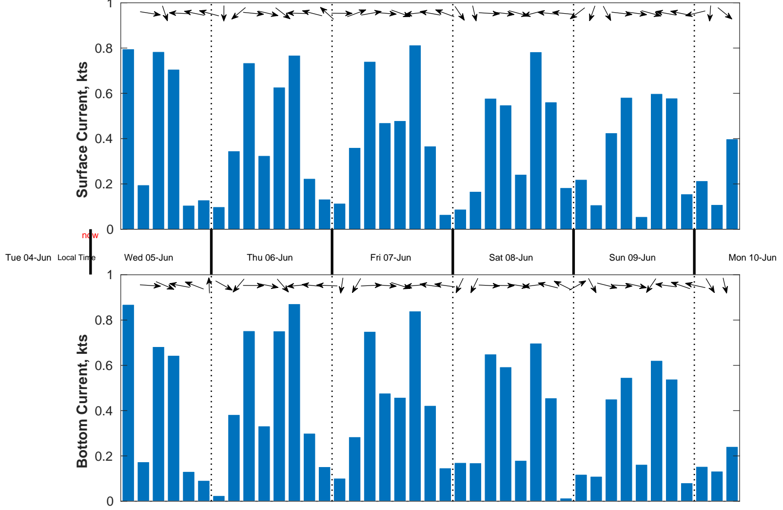
Surface Current Forecast for Targa Resources West Cameron GOM from 05-Jun-2024 21:00:00 to 11-Jun-2024 00:00:00
