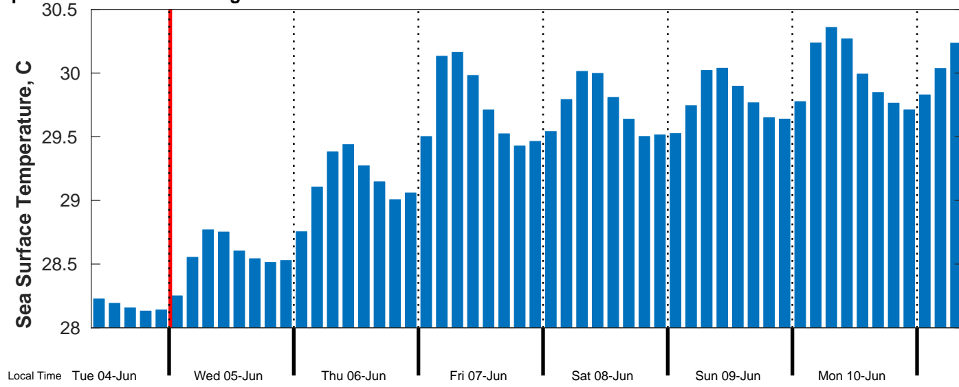
Sea Surface Temperature Forecast for Targa Resources West Cameron GOM from 05-Jun-2024 00:00:00 to 12-Jun-2024 00:00:00
