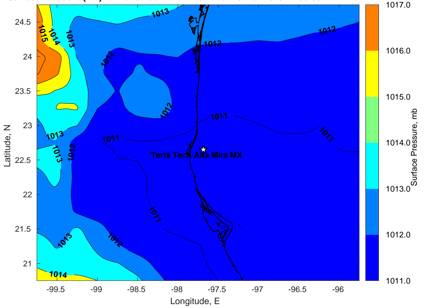
Surface Pressure (mb) for Terta Tech Alta Mira MX at 13-Mar-2023 12:00:00
