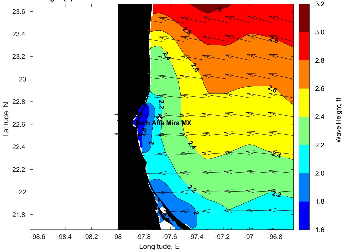
Wave Height (ft) for Terta Tech Alta Mira MX at 11-Mar-2023 12:00:00
