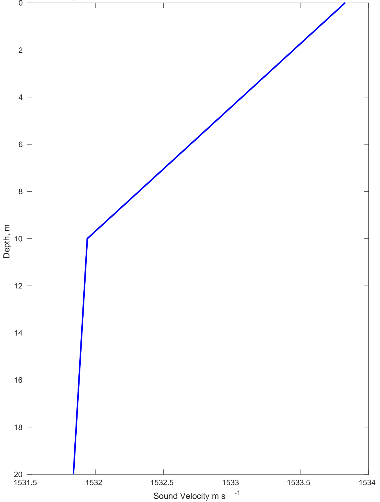
Sound Velocity Profile for Terta Tech Alta Mira MX on 11-Mar-2023 00:00:00
