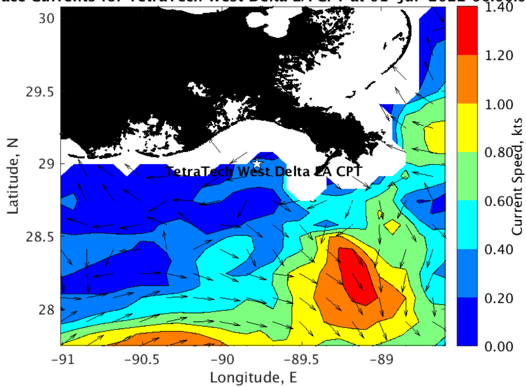
face Currents for TetraTech West Delta LA CPT at 01-Jul-2022 00:00:00
