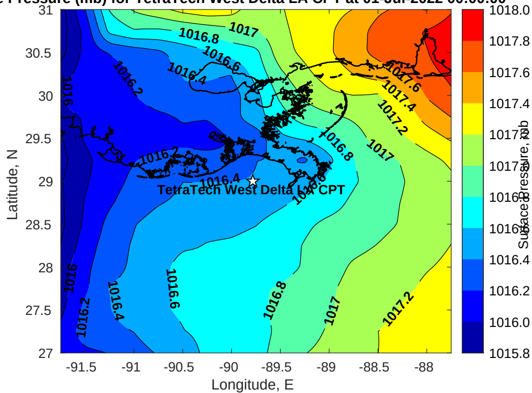
Surface Pressure (mb) for TetraTech West Delta LA CPT at 01-Jul-2022 00:00:00
