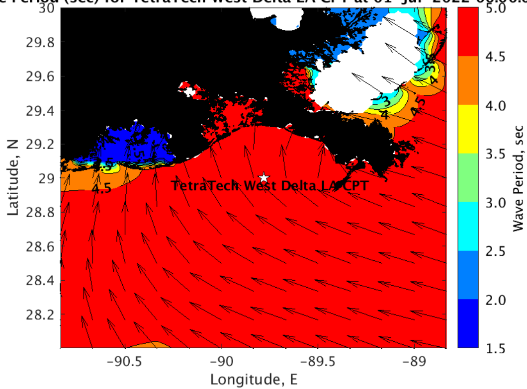
Wave Period (sec) for TetraTech West Delta LA CPT at 01-Jul-2022 00:00:00
