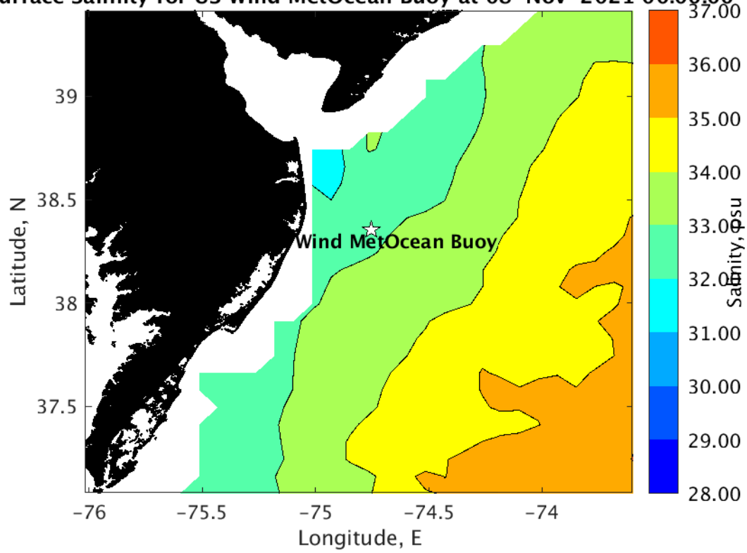
Surface Salinity for US Wind MetOcean Buoy at 08-Nov-2021 00:00:00
