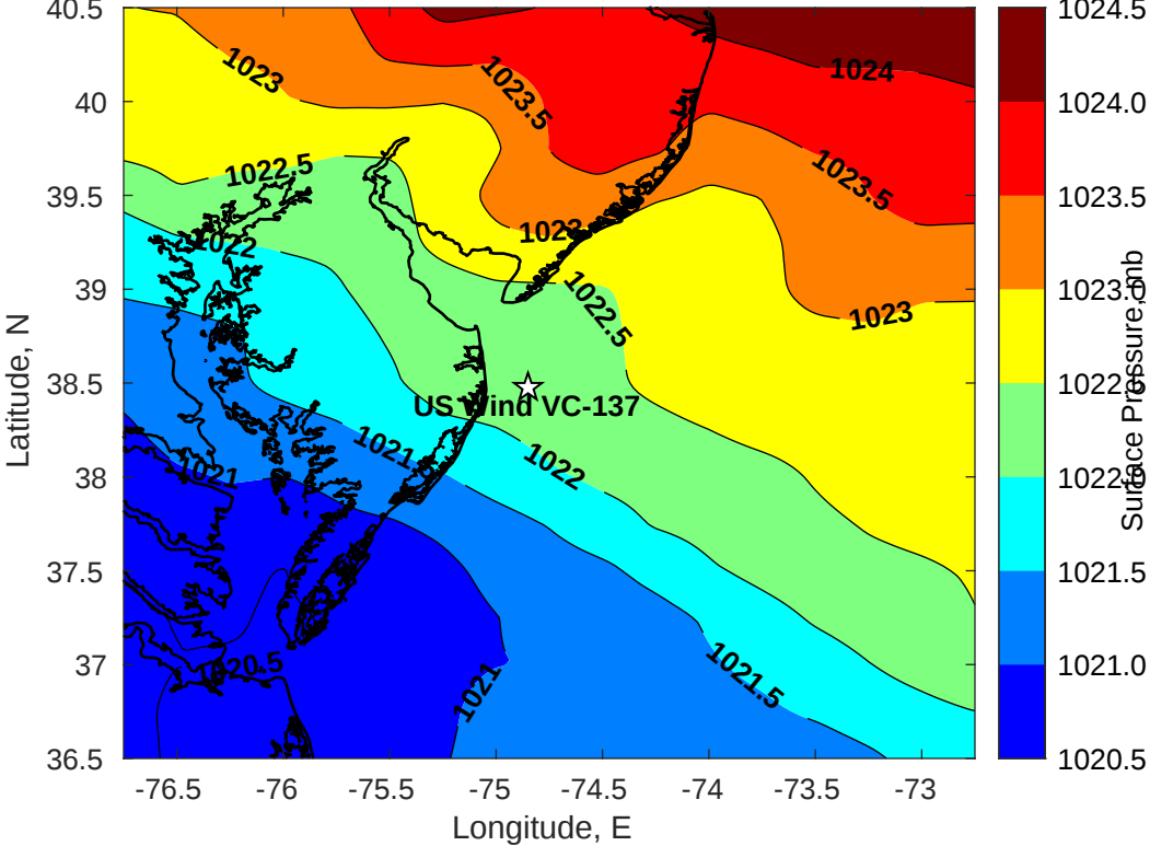
Surface Pressure (mb) for US Wind VC-137 at 23-Mar-2022 06:00:00
