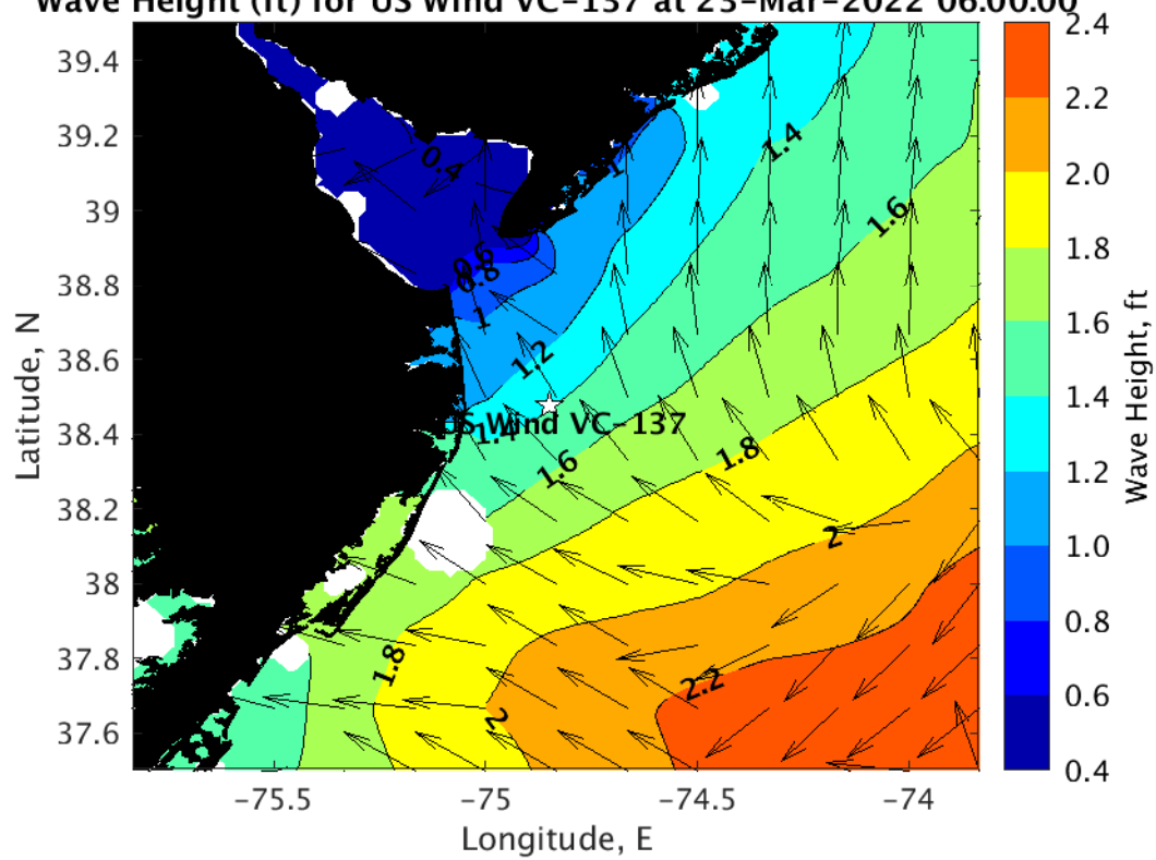
Wave Height (ft) for US Wind VC-137 at 23-Mar-2022 06:00:00
