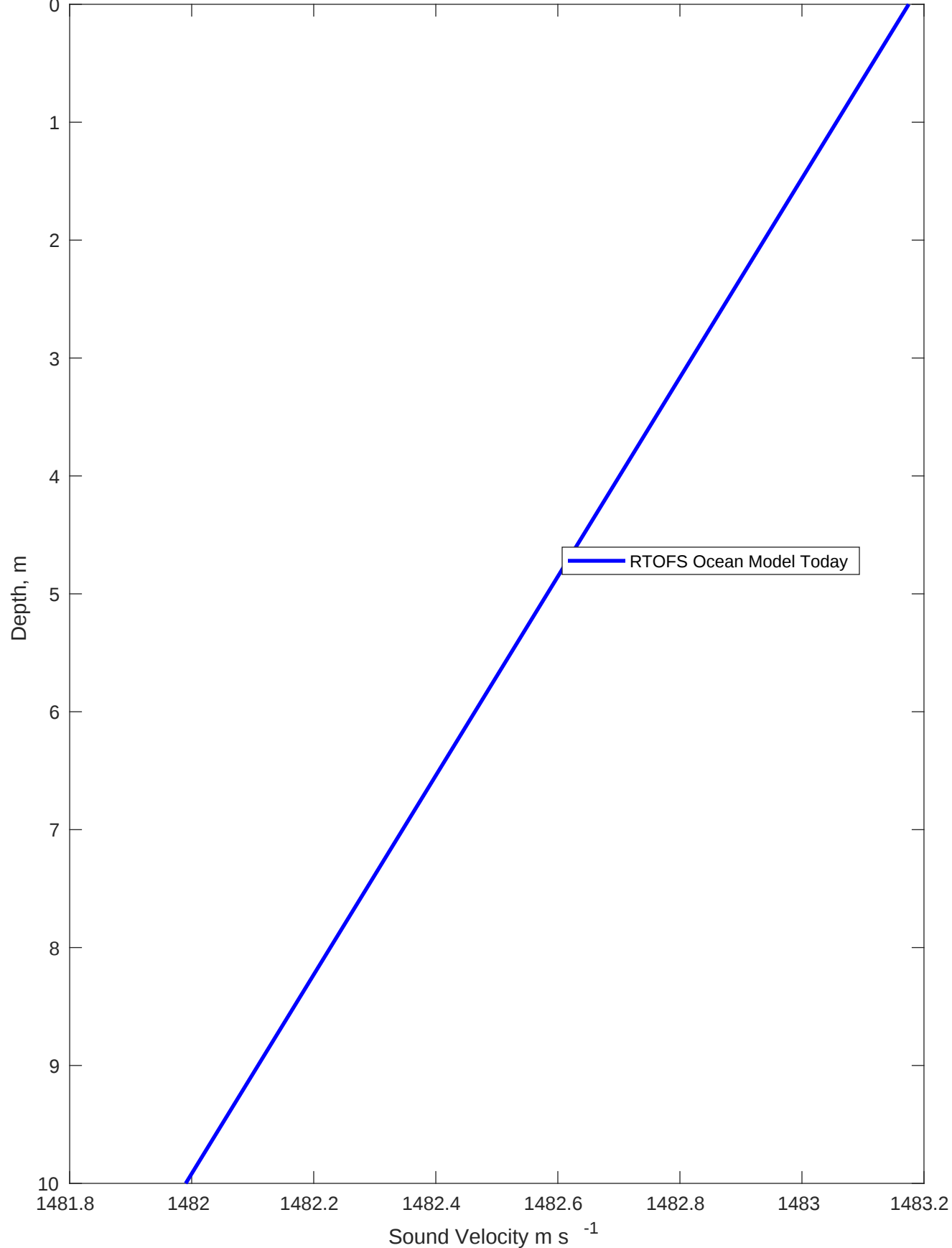
Sound Velocity Profile for US Wind VC-137 on 23-Mar-2022 00:00:00
