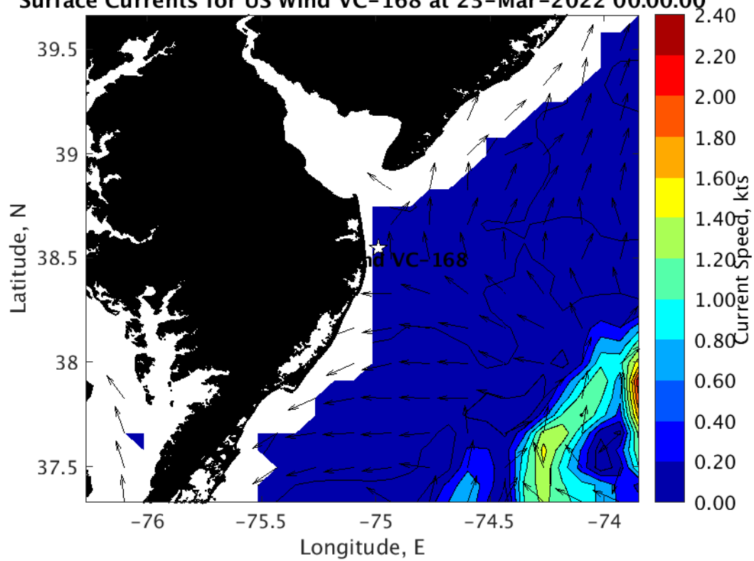
Surface Currents for US Wind VC-168 at 23-Mar-2022 00:00:00
