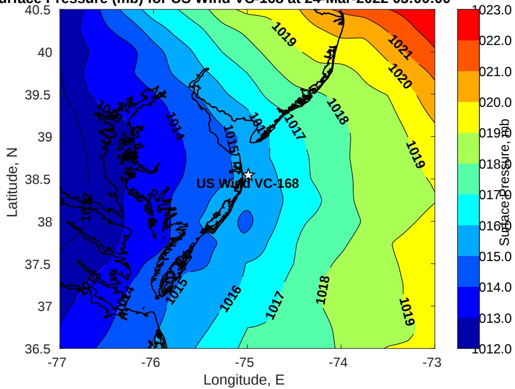
Surface Pressure (mb) for US Wind VC-168 at 24-Mar-2022 03:00:00
