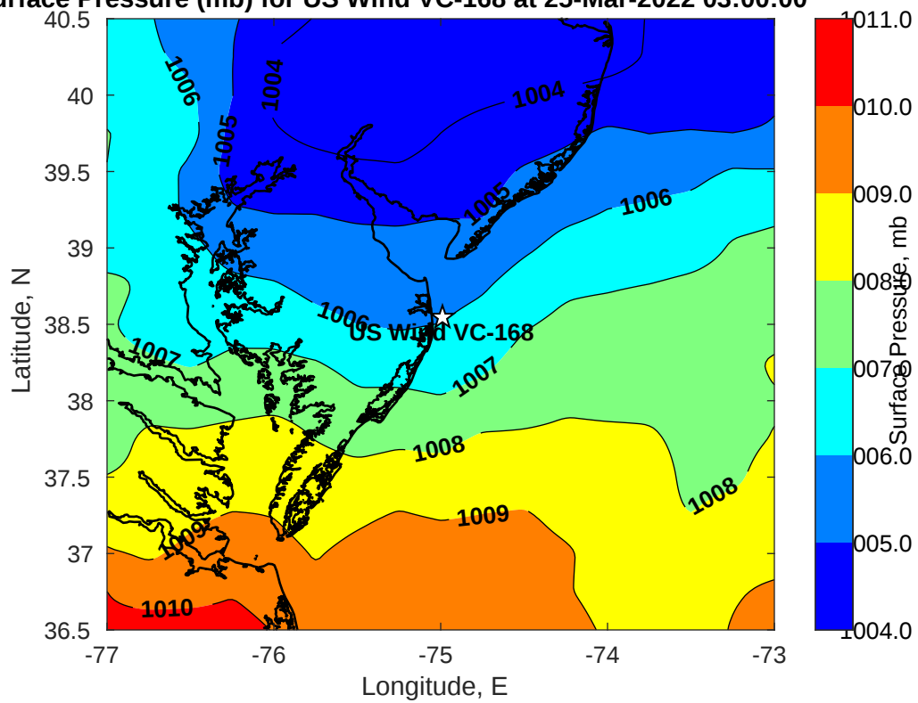
Surface Pressure (mb) for US Wind VC-168 at 25-Mar-2022 03:00:00
