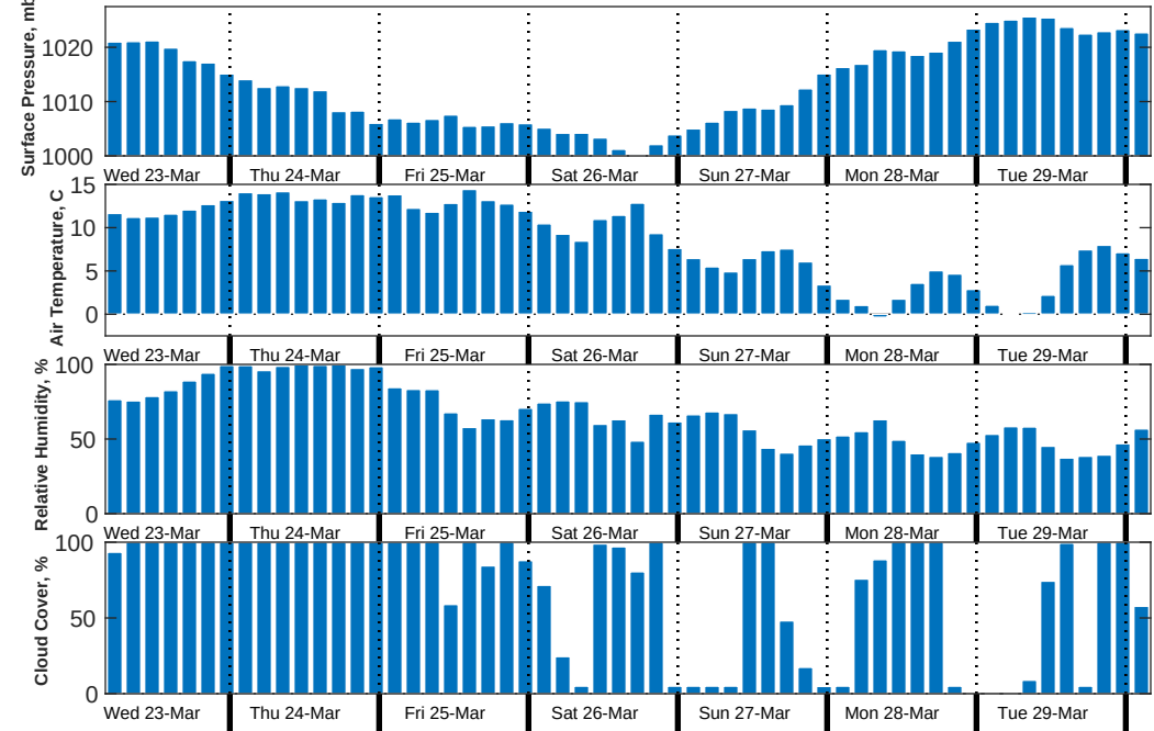
Met Forecast for US Wind VC-168 from 23-Mar-2022 06:00:00 to 30-Mar-2022 06:00:00
