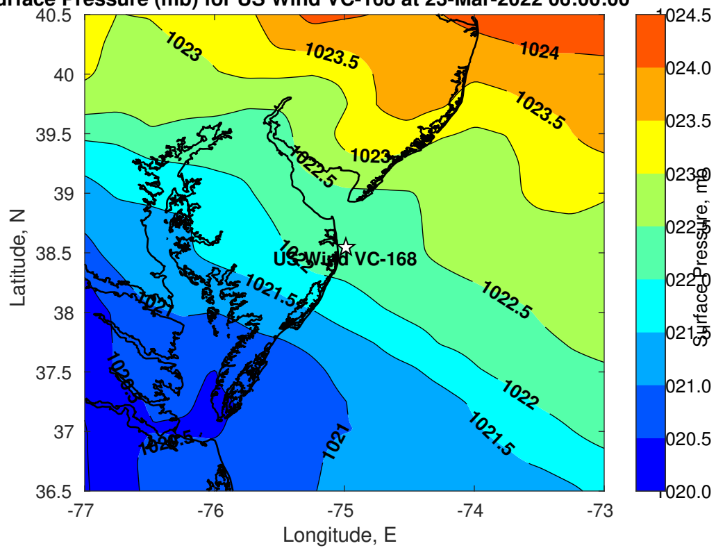
Surface Pressure (mb) for US Wind VC-168 at 23-Mar-2022 06:00:00
