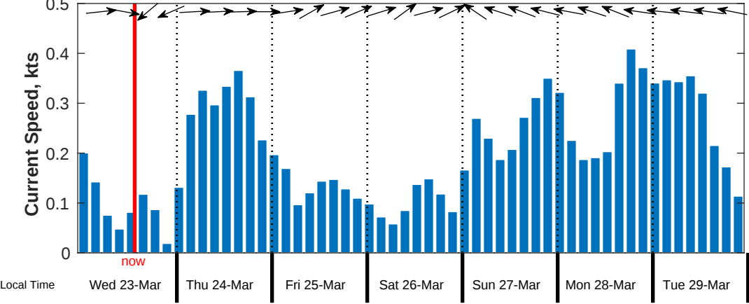
Current Forecast for US Wind VC-168 from 23-Mar-2022 00:00:00 to 30-Mar-2022 00:00:00
