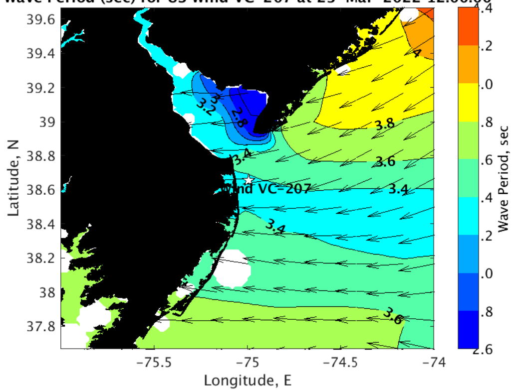
Wave Period (sec) for US Wind VC-207 at 23-Mar-2022 12:00:00
